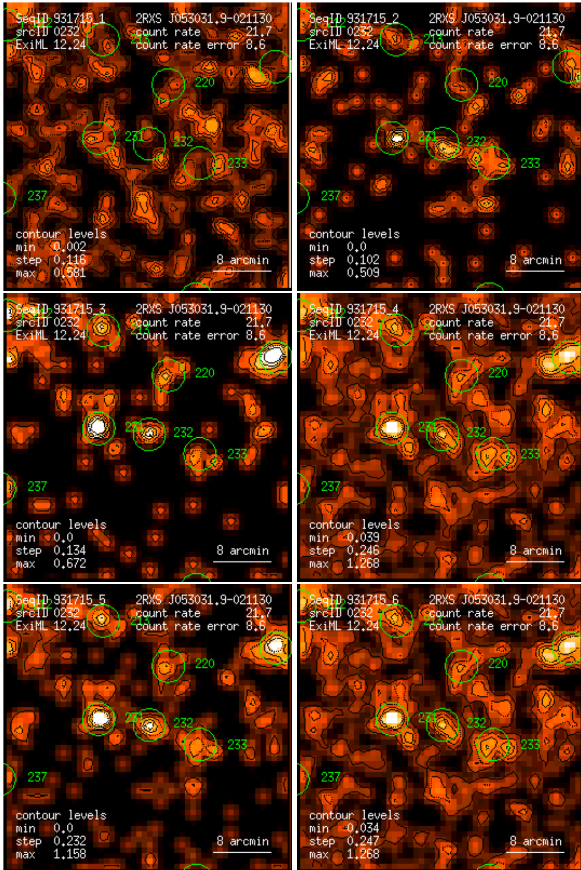
Figure 232: RASS 931715: detection 0232: band rate images, Gaussian filter: (1) PSPC channels 11 – 41, (2) 52 – 90, (3) 91 – 201, (4) 11 – 235, (5) 52 – 201, (6) 11 – 201. Broad band rates in counts/ks. Band rate contour levels in counts/ks/arcmin 2 .
