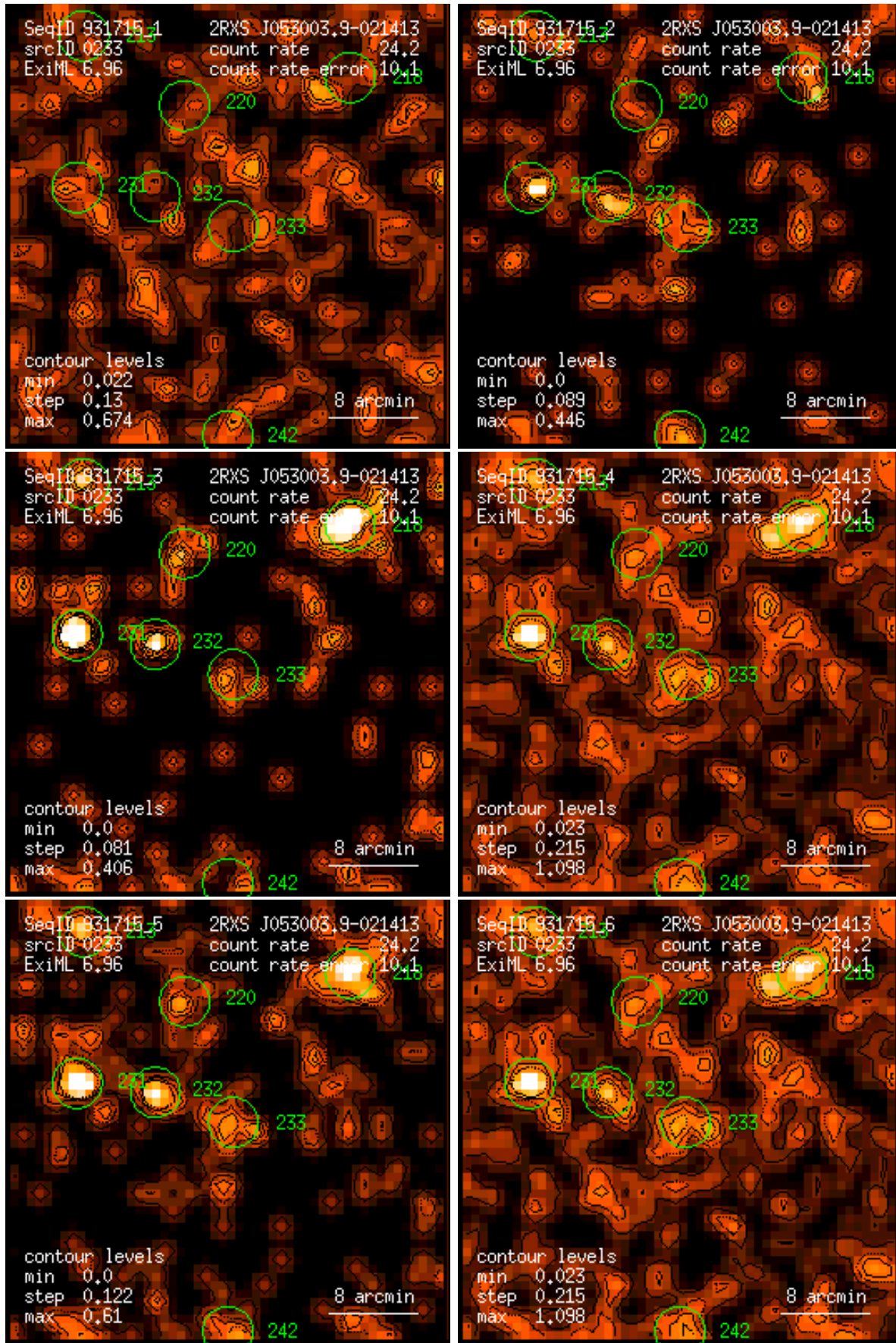
Figure 233: RASS 931715: detection 0233: band rate images, Gaussian filter: (1) PSPC channels 11 – 41, (2) 52 – 90, (3) 91 – 201, (4) 11 – 235, (5) 52 – 201, (6) 11 – 201. Broad band rates in counts/ks. Band rate contour levels in counts/ks/arcmin 2 .
