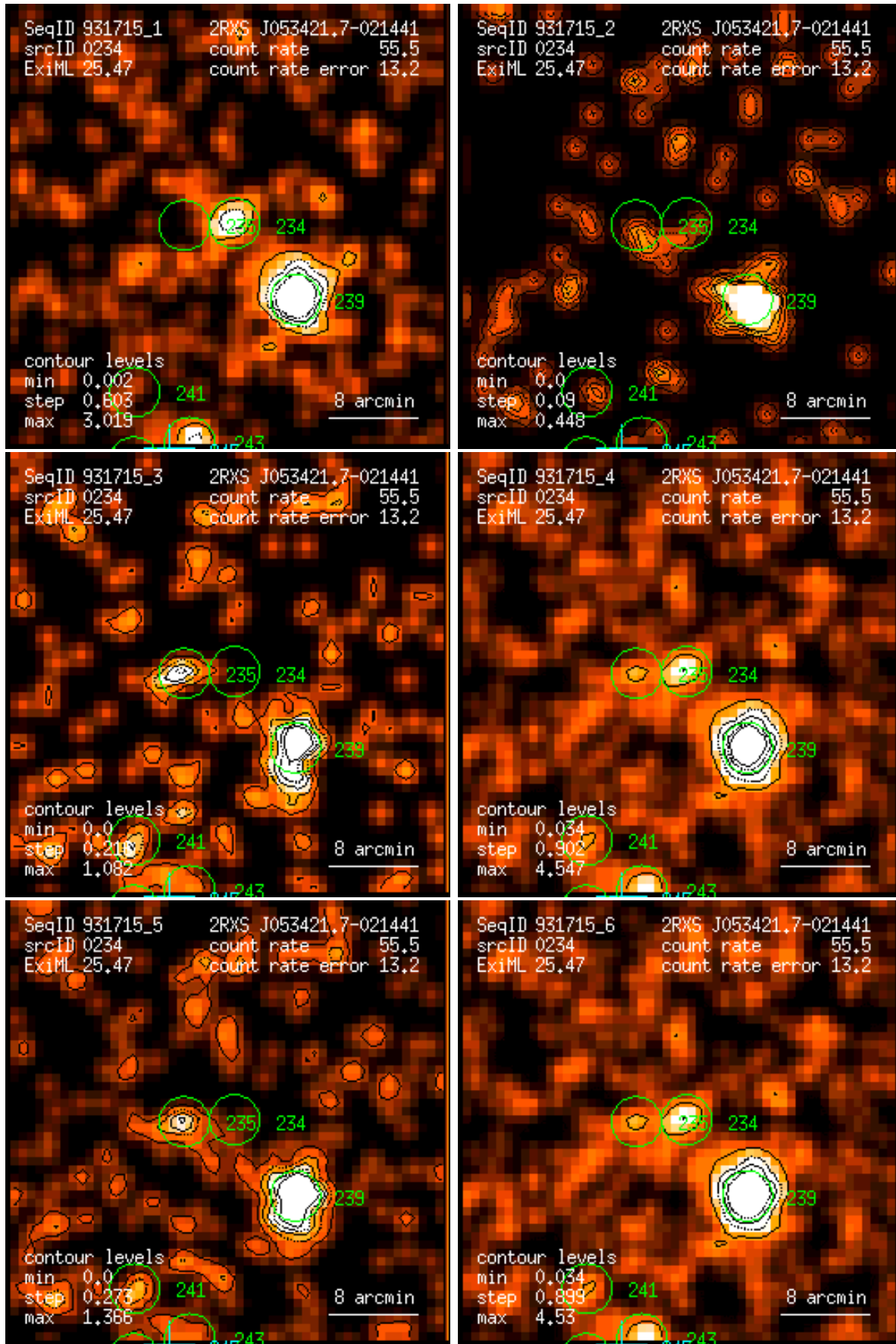
Figure 234: RASS 931715: detection 0234: band rate images, Gaussian filter: (1) PSPC channels 11 – 41, (2) 52 – 90, (3) 91 – 201, (4) 11 – 235, (5) 52 – 201, (6) 11 – 201. Broad band rates in counts/ks. Band rate contour levels in counts/ks/arcmin 2 .
