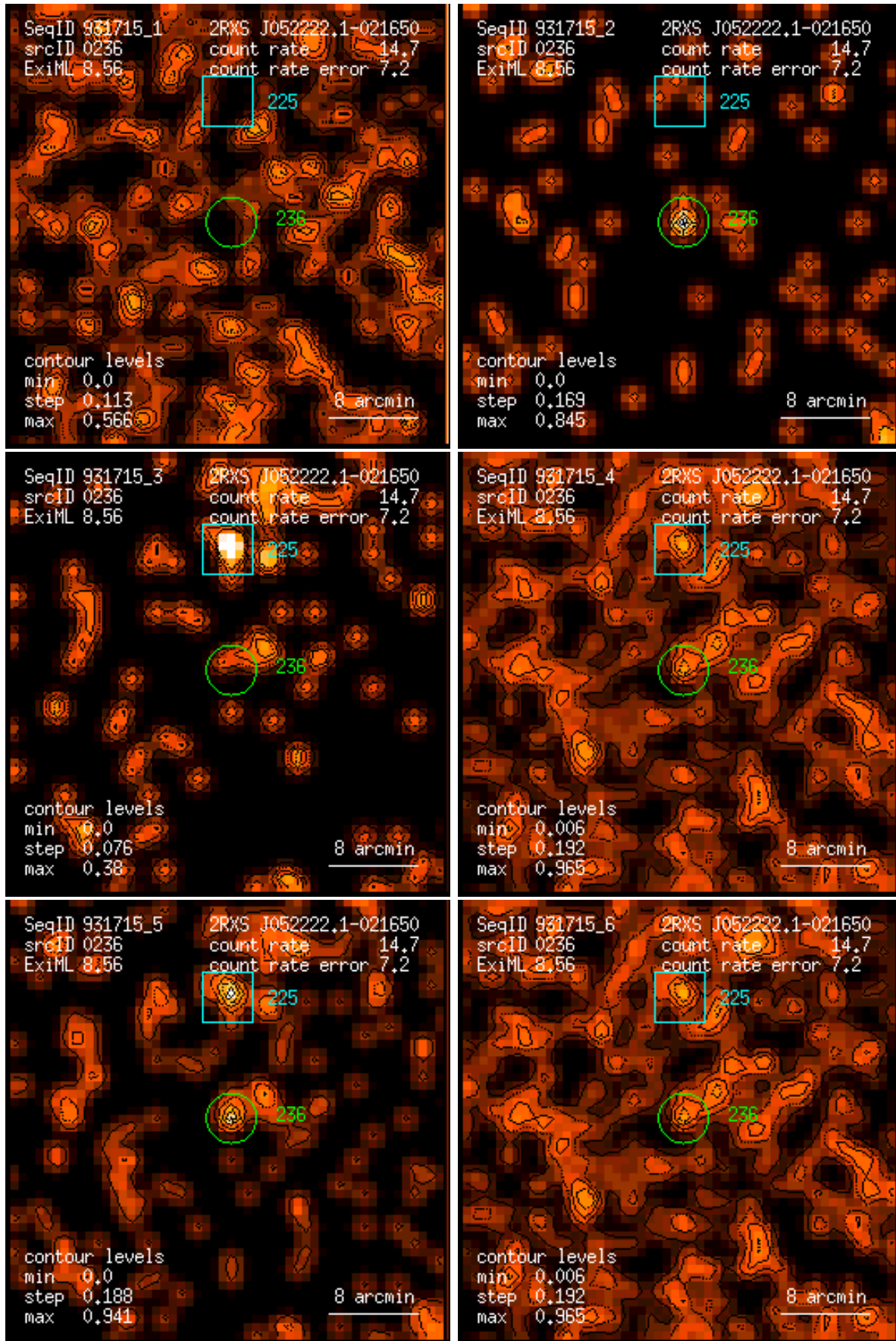
Figure 236: RASS 931715: detection 0236: band rate images, Gaussian filter: (1) PSPC channels 11 – 41, (2) 52 – 90, (3) 91 – 201, (4) 11 – 235, (5) 52 – 201, (6) 11 – 201. Broad band rates in counts/ks. Band rate contour levels in counts/ks/arcmin 2 .
