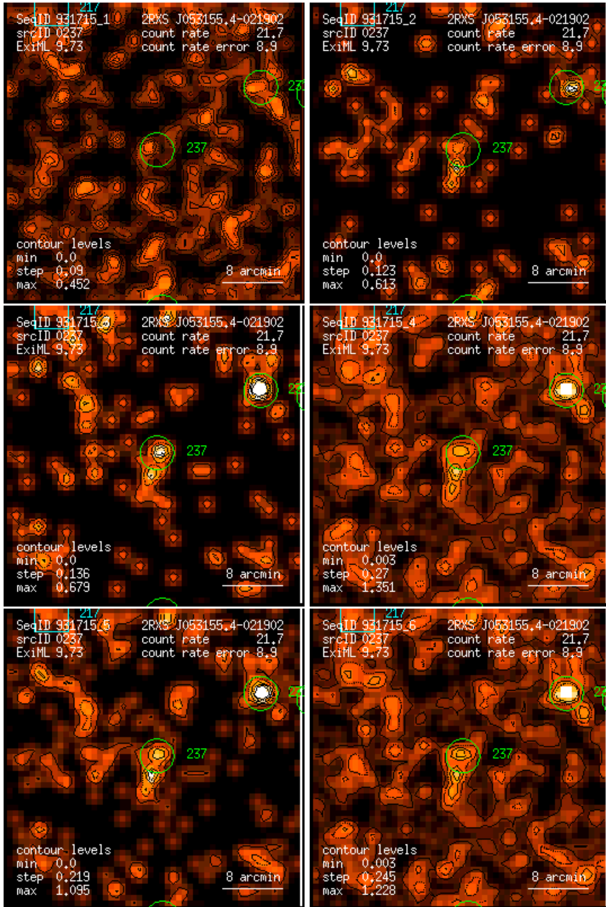
Figure 237: RASS 931715: detection 0237: band rate images, Gaussian filter: (1) PSPC channels 11 – 41, (2) 52 – 90, (3) 91 – 201, (4) 11 – 235, (5) 52 – 201, (6) 11 – 201. Broad band rates in counts/ks. Band rate contour levels in counts/ks/arcmin 2 .
