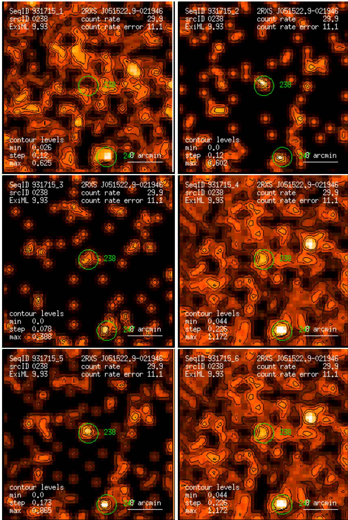
Figure 238: RASS 931715: detection 0238: band rate images, Gaussian filter: (1) PSPC channels 11 – 41, (2) 52 – 90, (3) 91 – 201, (4) 11 – 235, (5) 52 – 201, (6) 11 – 201. Broad band rates in counts/ks. Band rate contour levels in counts/ks/arcmin 2 .
