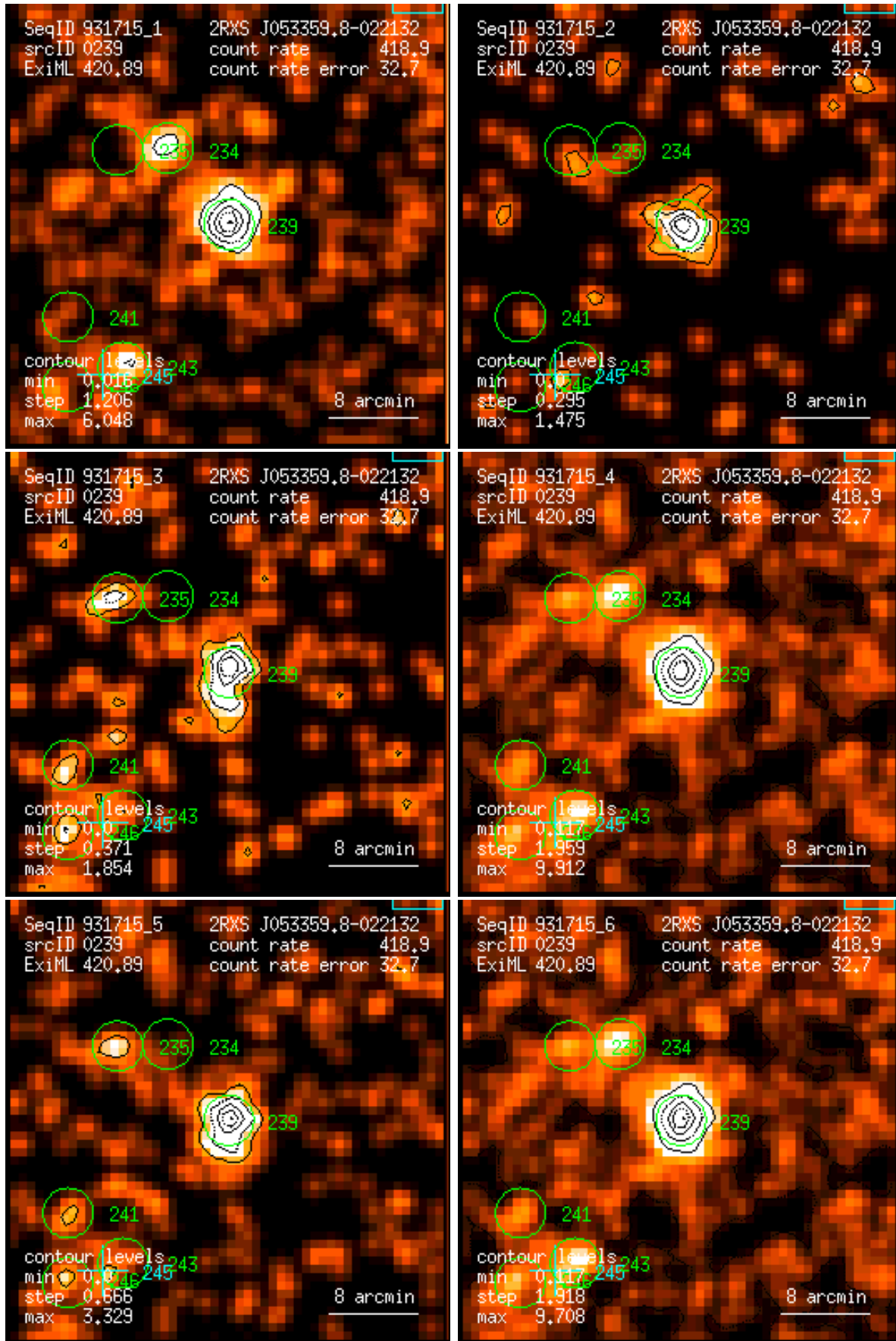
Figure 239: RASS 931715: detection 0239: band rate images, Gaussian filter: (1) PSPC channels 11 – 41, (2) 52 – 90, (3) 91 – 201, (4) 11 – 235, (5) 52 – 201, (6) 11 – 201. Broad band rates in counts/ks. Band rate contour levels in counts/ks/arcmin 2 .
