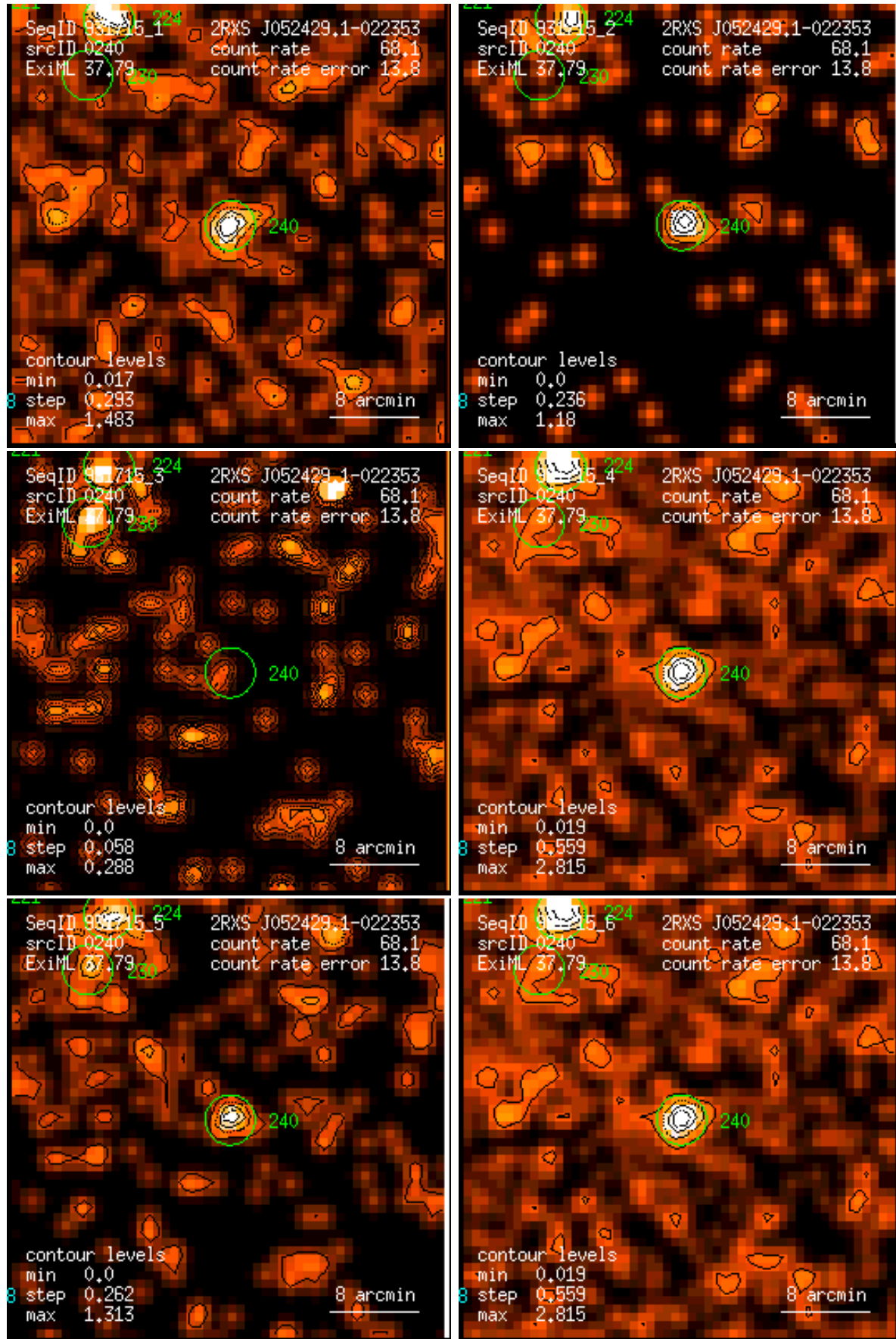
Figure 240: RASS 931715: detection 0240: band rate images, Gaussian filter: (1) PSPC channels 11 – 41, (2) 52 – 90, (3) 91 – 201, (4) 11 – 235, (5) 52 – 201, (6) 11 – 201. Broad band rates in counts/ks. Band rate contour levels in counts/ks/arcmin 2 .
