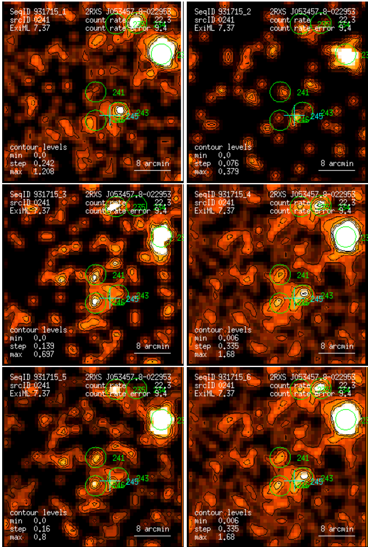
Figure 241: RASS 931715: detection 0241: band rate images, Gaussian filter: (1) PSPC channels 11 – 41, (2) 52 – 90, (3) 91 – 201, (4) 11 – 235, (5) 52 – 201, (6) 11 – 201. Broad band rates in counts/ks. Band rate contour levels in counts/ks/arcmin 2 .
