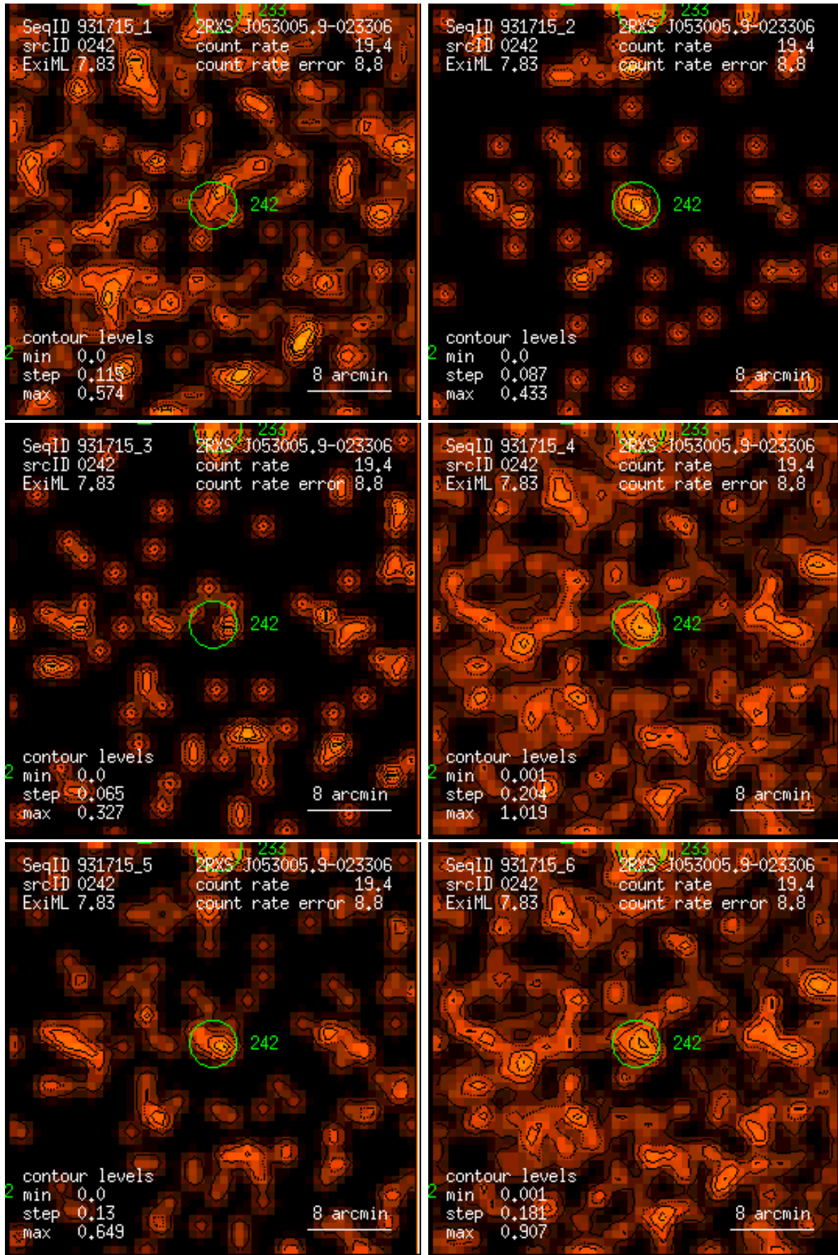
Figure 242: RASS 931715: detection 0242: band rate images, Gaussian filter: (1) PSPC channels 11 – 41, (2) 52 – 90, (3) 91 – 201, (4) 11 – 235, (5) 52 – 201, (6) 11 – 201. Broad band rates in counts/ks. Band rate contour levels in counts/ks/arcmin 2 .
