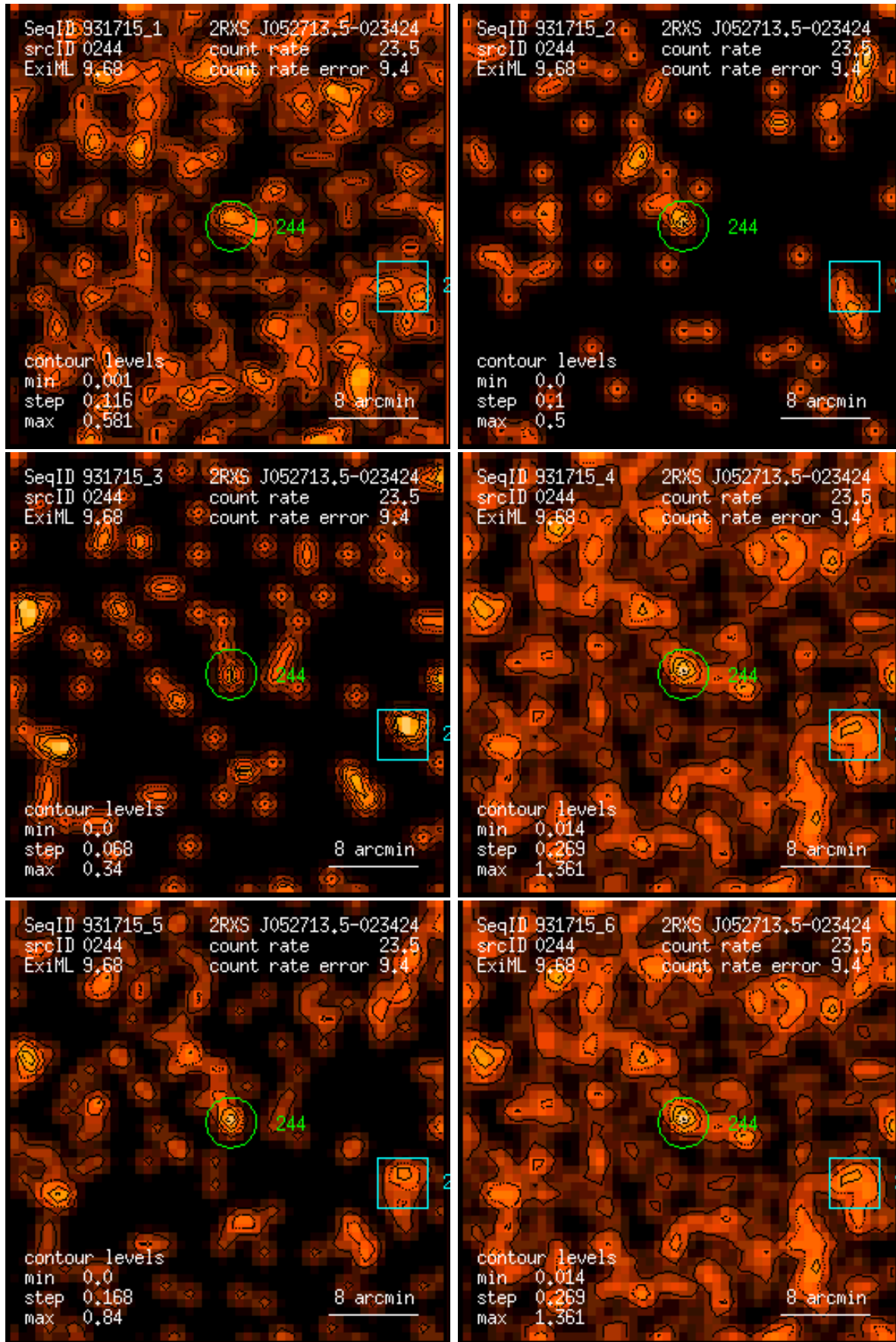
Figure 244: RASS 931715: detection 0244: band rate images, Gaussian filter: (1) PSPC channels 11 – 41, (2) 52 – 90, (3) 91 – 201, (4) 11 – 235, (5) 52 – 201, (6) 11 – 201. Broad band rates in counts/ks. Band rate contour levels in counts/ks/arcmin 2 .
