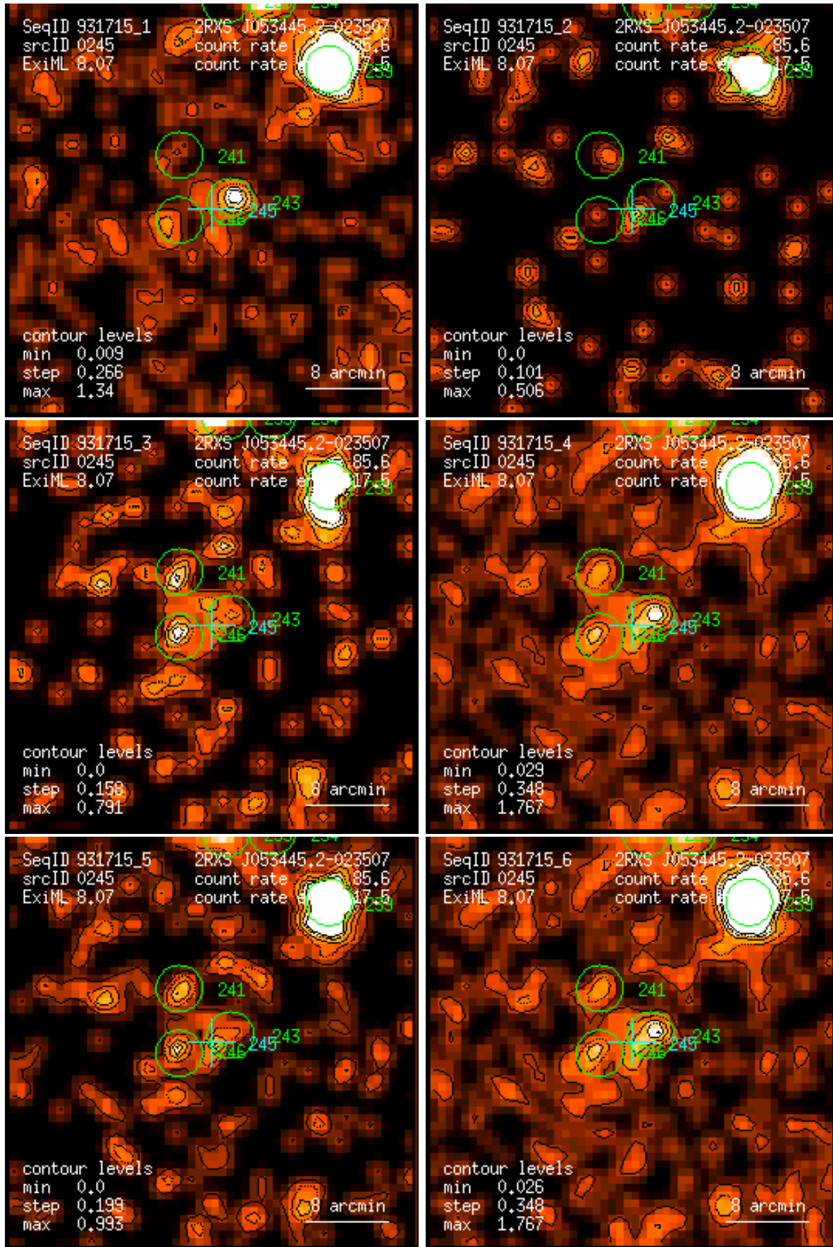
Figure 245: RASS 931715: detection 0245: band rate images, Gaussian filter: (1) PSPC channels 11 – 41, (2) 52 – 90, (3) 91 – 201, (4) 11 – 235, (5) 52 – 201, (6) 11 – 201. Broad band rates in counts/ks. Band rate contour levels in counts/ks/arcmin 2 .
