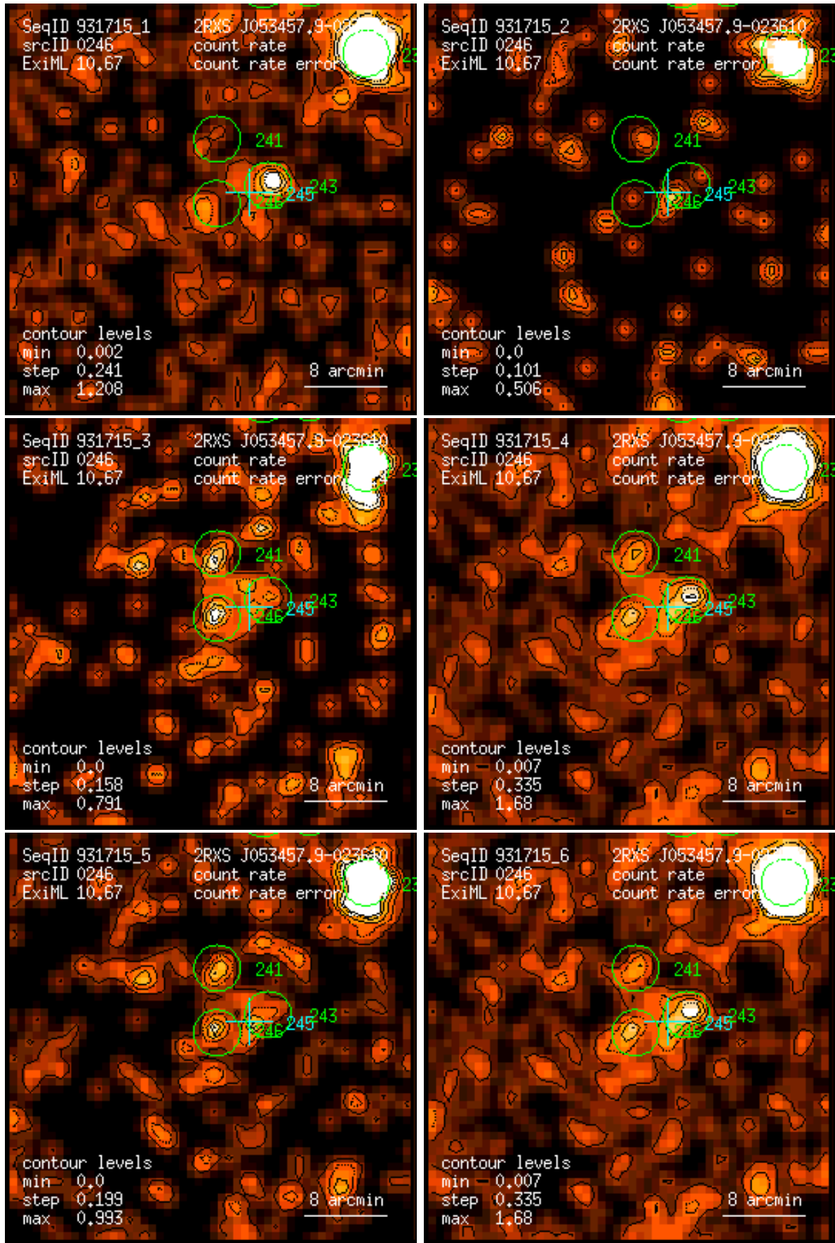
Figure 246: RASS 931715: detection 0246: band rate images, Gaussian filter: (1) PSPC channels 11 – 41, (2) 52 – 90, (3) 91 – 201, (4) 11 – 235, (5) 52 – 201, (6) 11 – 201. Broad band rates in counts/ks. Band rate contour levels in counts/ks/arcmin 2 .
