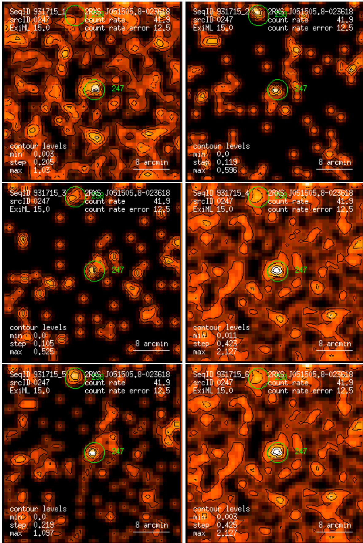
Figure 247: RASS 931715: detection 0247: band rate images, Gaussian filter: (1) PSPC channels 11 – 41, (2) 52 – 90, (3) 91 – 201, (4) 11 – 235, (5) 52 – 201, (6) 11 – 201. Broad band rates in counts/ks. Band rate contour levels in counts/ks/arcmin 2 .
