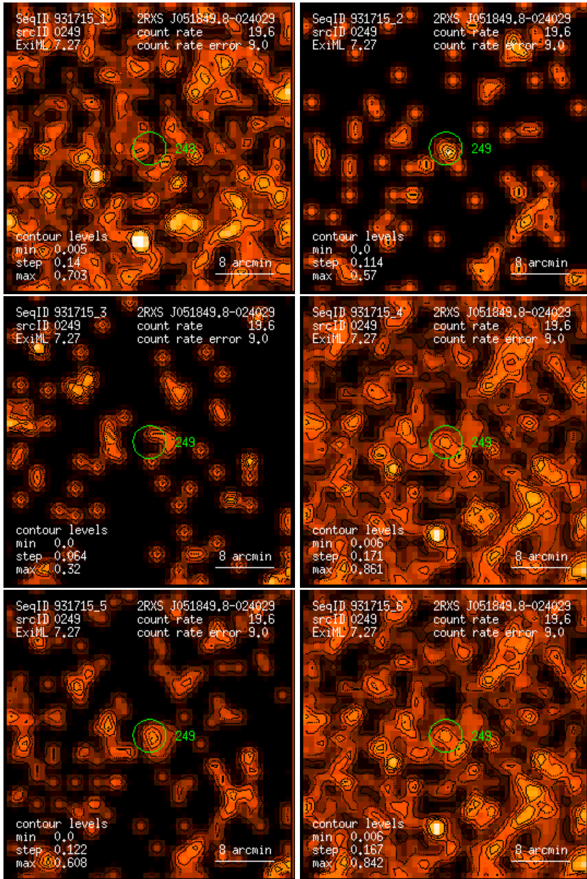
Figure 249: RASS 931715: detection 0249: band rate images, Gaussian filter: (1) PSPC channels 11 – 41, (2) 52 – 90, (3) 91 – 201, (4) 11 – 235, (5) 52 – 201, (6) 11 – 201. Broad band rates in counts/ks. Band rate contour levels in counts/ks/arcmin 2 .
