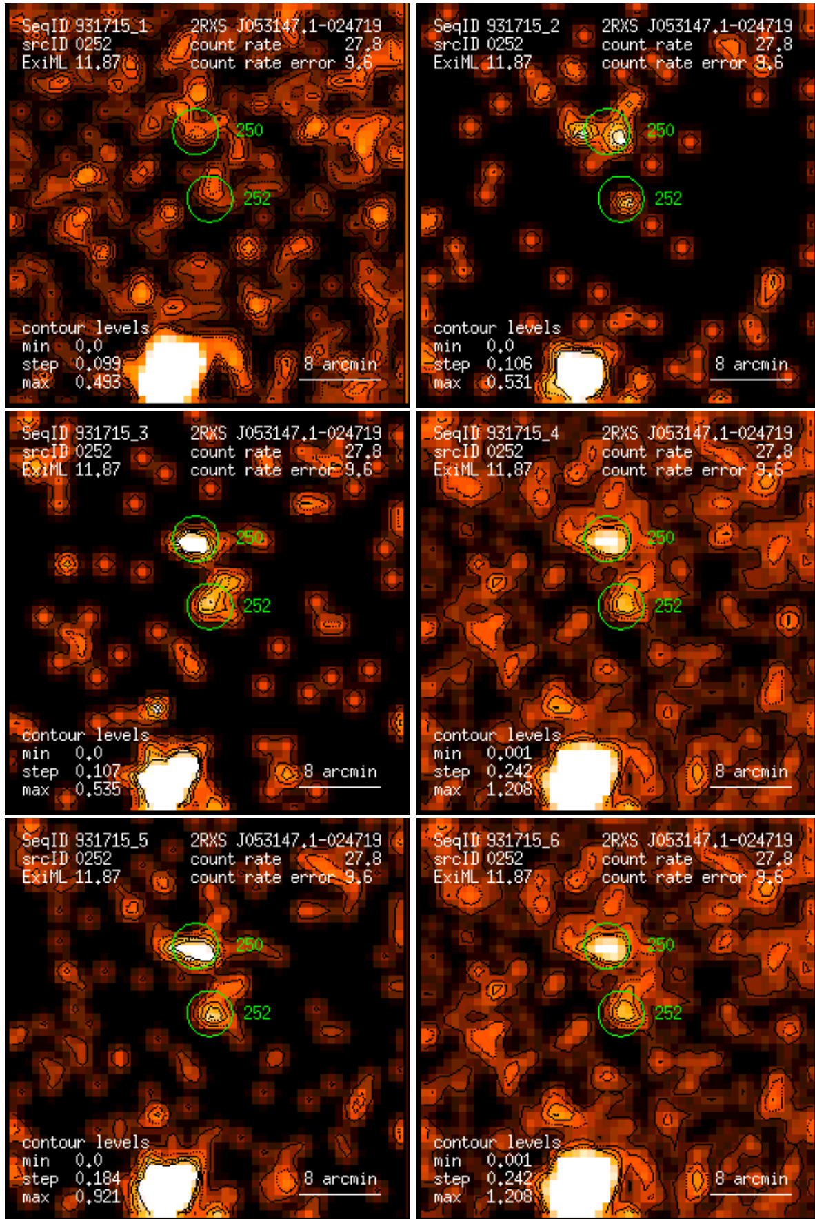
Figure 252: RASS 931715: detection 0252: band rate images, Gaussian filter: (1) PSPC channels 11 – 41, (2) 52 – 90, (3) 91 – 201, (4) 11 – 235, (5) 52 – 201, (6) 11 – 201. Broad band rates in counts/ks. Band rate contour levels in counts/ks/arcmin 2 .
