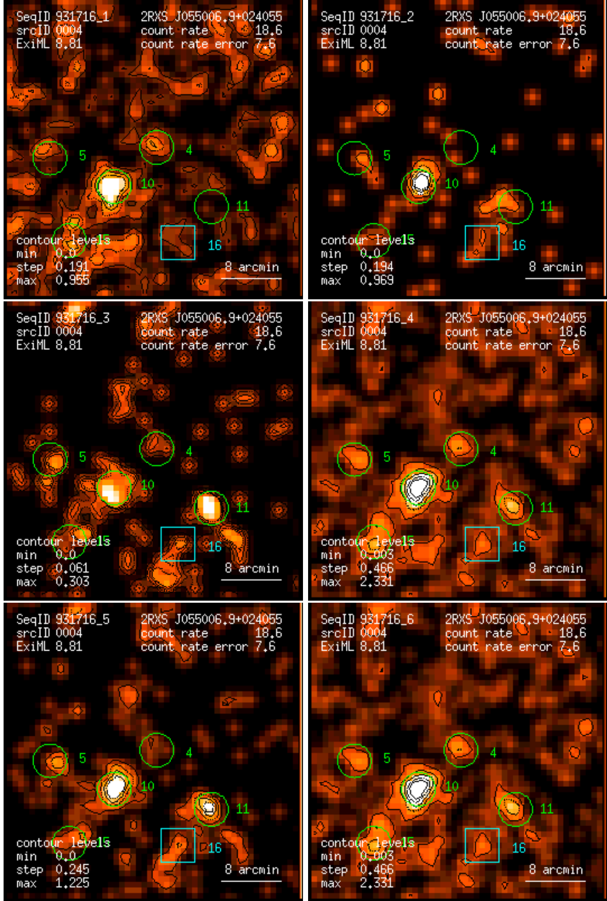
Figure 4: RASS 931716: detection 0004: band rate images, Gaussian filter: (1) PSPC channels 11 – 41, (2) 52 – 90, (3) 91 – 201, (4) 11 – 235, (5) 52 – 201, (6) 11 – 201. Broad band rates in counts/ks. Band rate contour levels in counts/ks/arcmin 2 .
