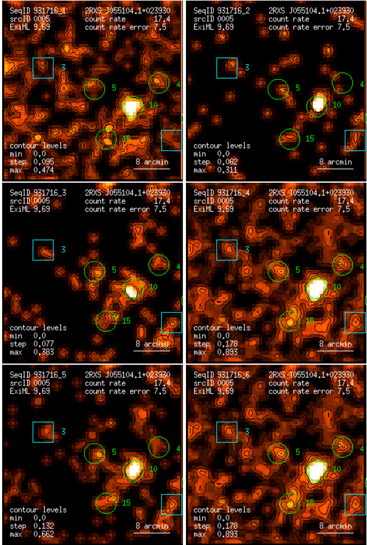
Figure 5: RASS 931716: detection 0005: band rate images, Gaussian filter: (1) PSPC channels 11 – 41, (2) 52 – 90, (3) 91 – 201, (4) 11 – 235, (5) 52 – 201, (6) 11 – 201. Broad band rates in counts/ks. Band rate contour levels in counts/ks/arcmin 2 .
