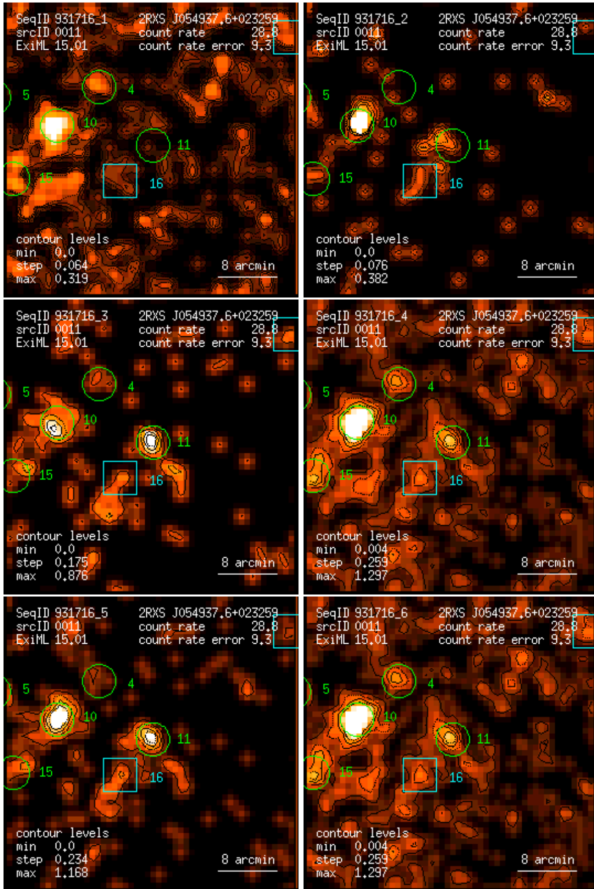
Figure 11: RASS 931716: detection 0011: band rate images, Gaussian filter: (1) PSPC channels 11 – 41, (2) 52 – 90, (3) 91 – 201, (4) 11 – 235, (5) 52 – 201, (6) 11 – 201. Broad band rates in counts/ks. Band rate contour levels in counts/ks/arcmin 2 .
