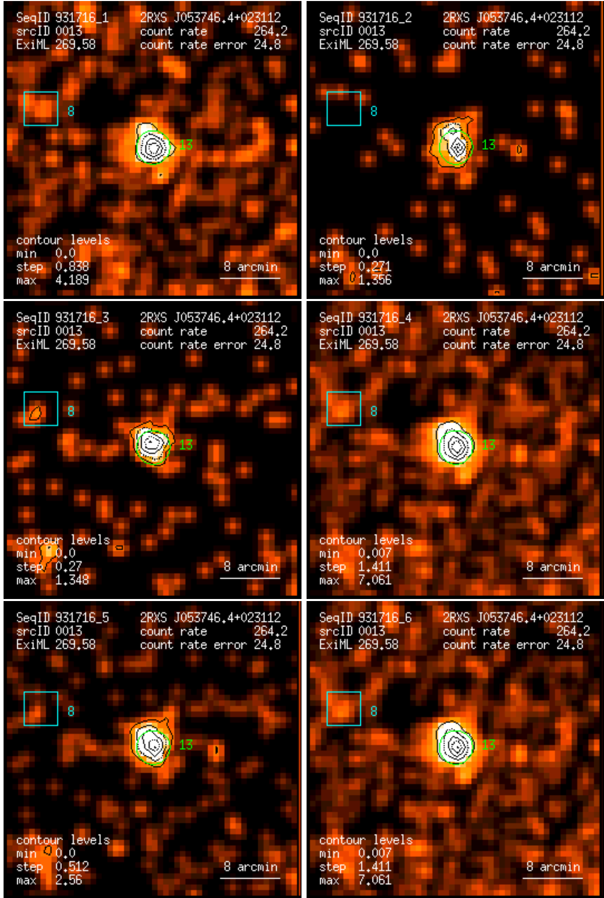
Figure 13: RASS 931716: detection 0013: band rate images, Gaussian filter: (1) PSPC channels 11 – 41, (2) 52 – 90, (3) 91 – 201, (4) 11 – 235, (5) 52 – 201, (6) 11 – 201. Broad band rates in counts/ks. Band rate contour levels in counts/ks/arcmin 2 .
