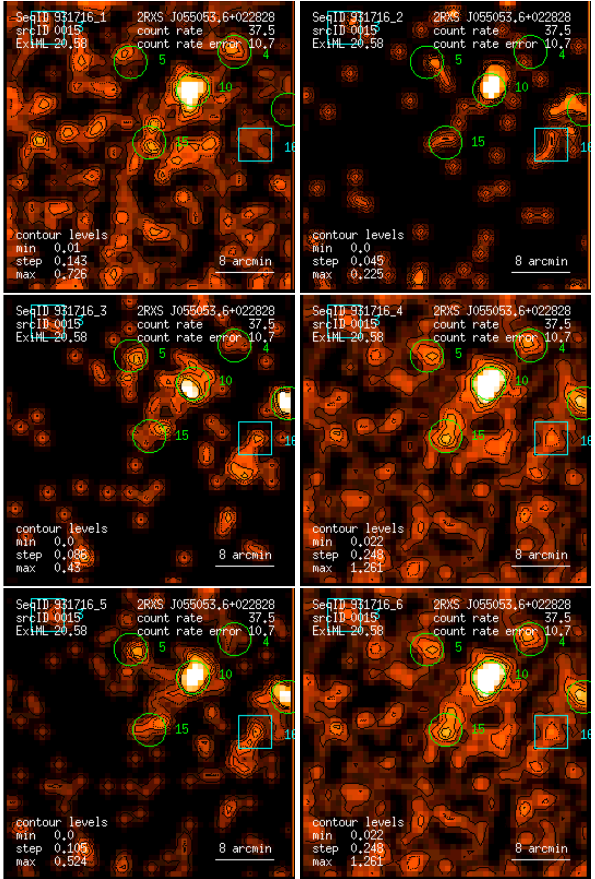
Figure 15: RASS 931716: detection 0015: band rate images, Gaussian filter: (1) PSPC channels 11 – 41, (2) 52 – 90, (3) 91 – 201, (4) 11 – 235, (5) 52 – 201, (6) 11 – 201. Broad band rates in counts/ks. Band rate contour levels in counts/ks/arcmin 2 .
