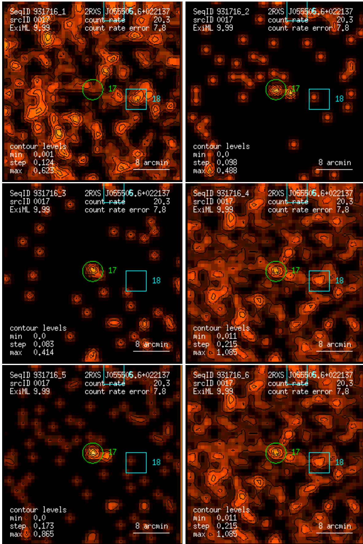
Figure 17: RASS 931716: detection 0017: band rate images, Gaussian filter: (1) PSPC channels 11 – 41, (2) 52 – 90, (3) 91 – 201, (4) 11 – 235, (5) 52 – 201, (6) 11 – 201. Broad band rates in counts/ks. Band rate contour levels in counts/ks/arcmin 2 .
