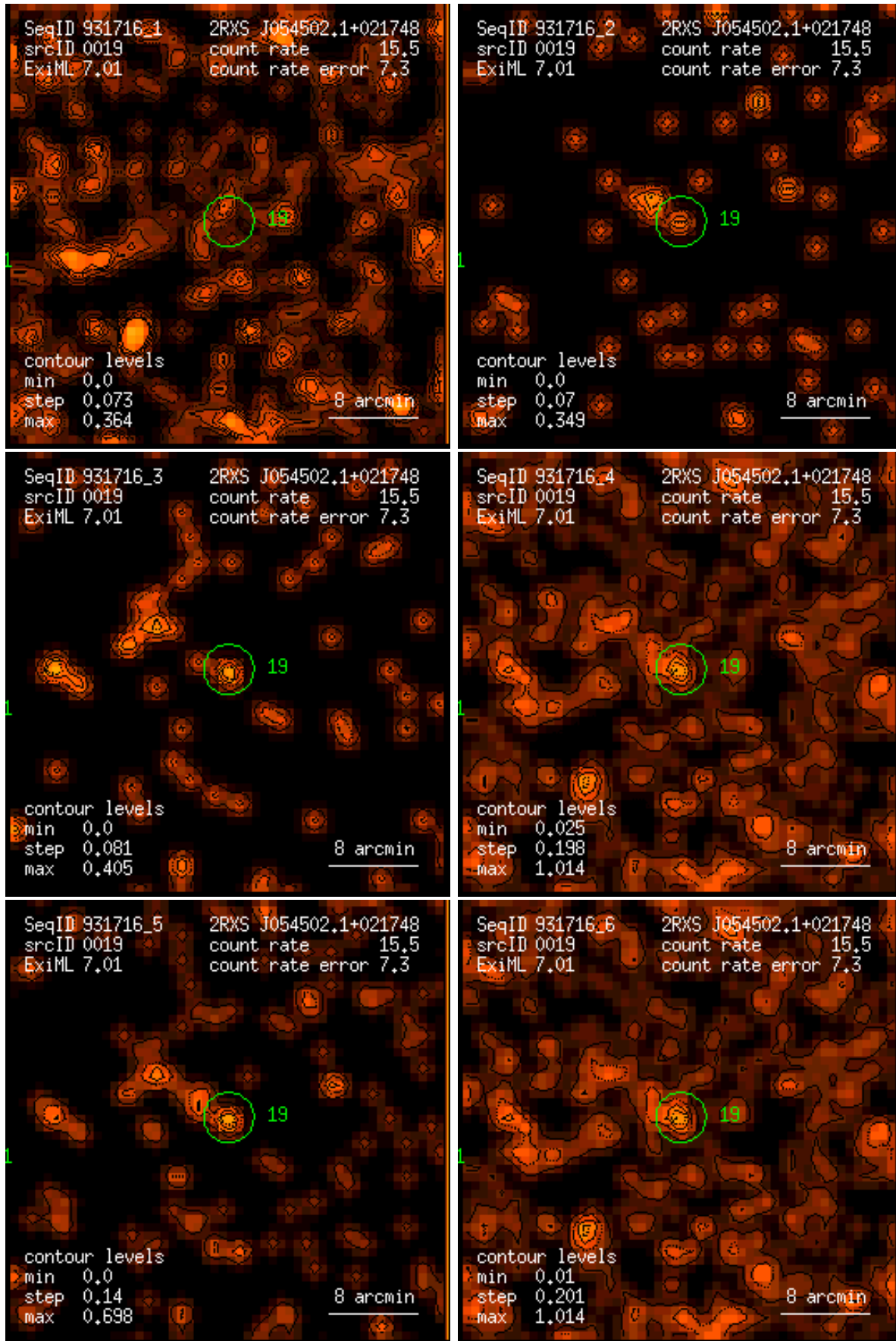
Figure 19: RASS 931716: detection 0019: band rate images, Gaussian filter: (1) PSPC channels 11 – 41, (2) 52 – 90, (3) 91 – 201, (4) 11 – 235, (5) 52 – 201, (6) 11 – 201. Broad band rates in counts/ks. Band rate contour levels in counts/ks/arcmin 2 .
