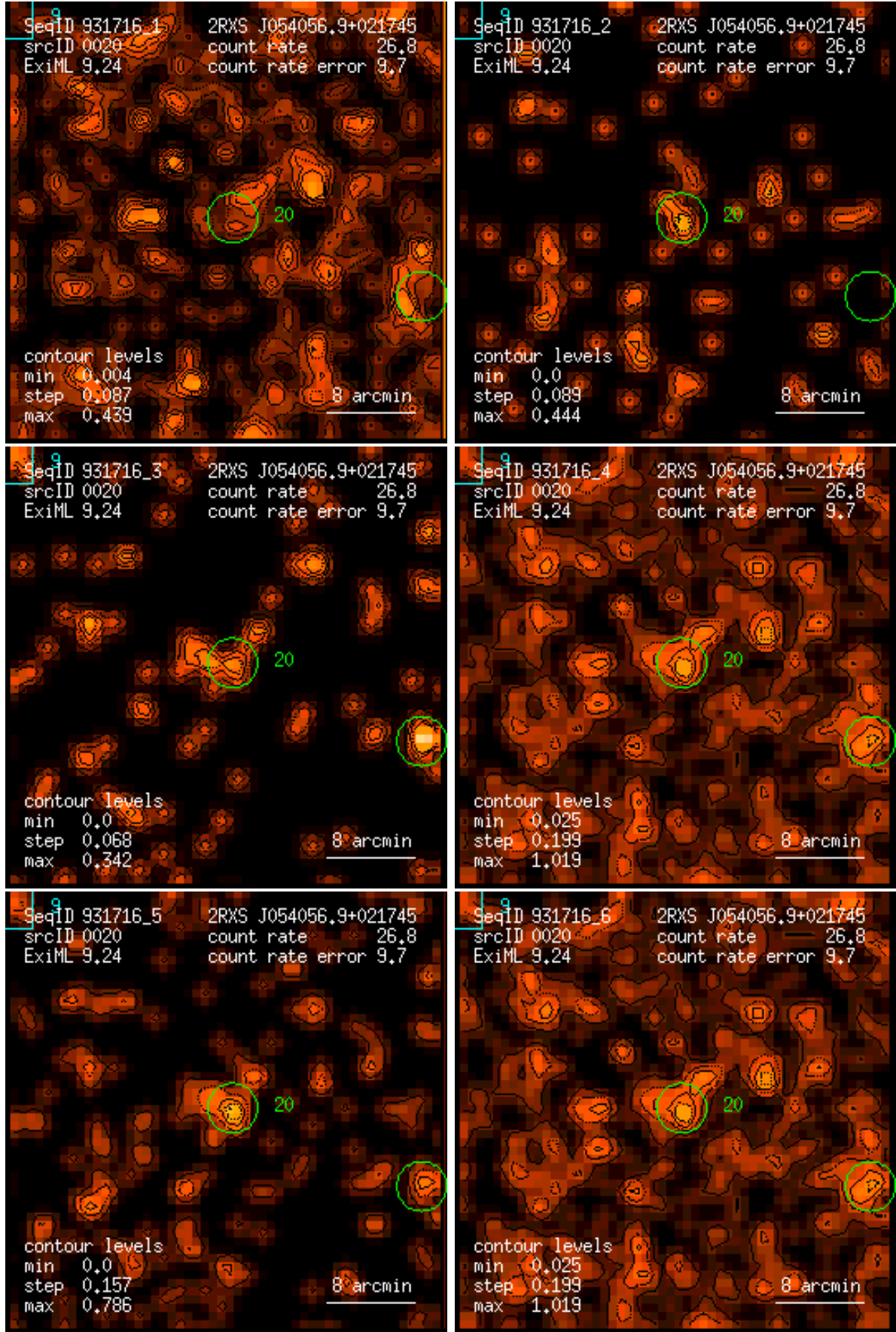
Figure 20: RASS 931716: detection 0020: band rate images, Gaussian filter: (1) PSPC channels 11 – 41, (2) 52 – 90, (3) 91 – 201, (4) 11 – 235, (5) 52 – 201, (6) 11 – 201. Broad band rates in counts/ks. Band rate contour levels in counts/ks/arcmin 2 .
