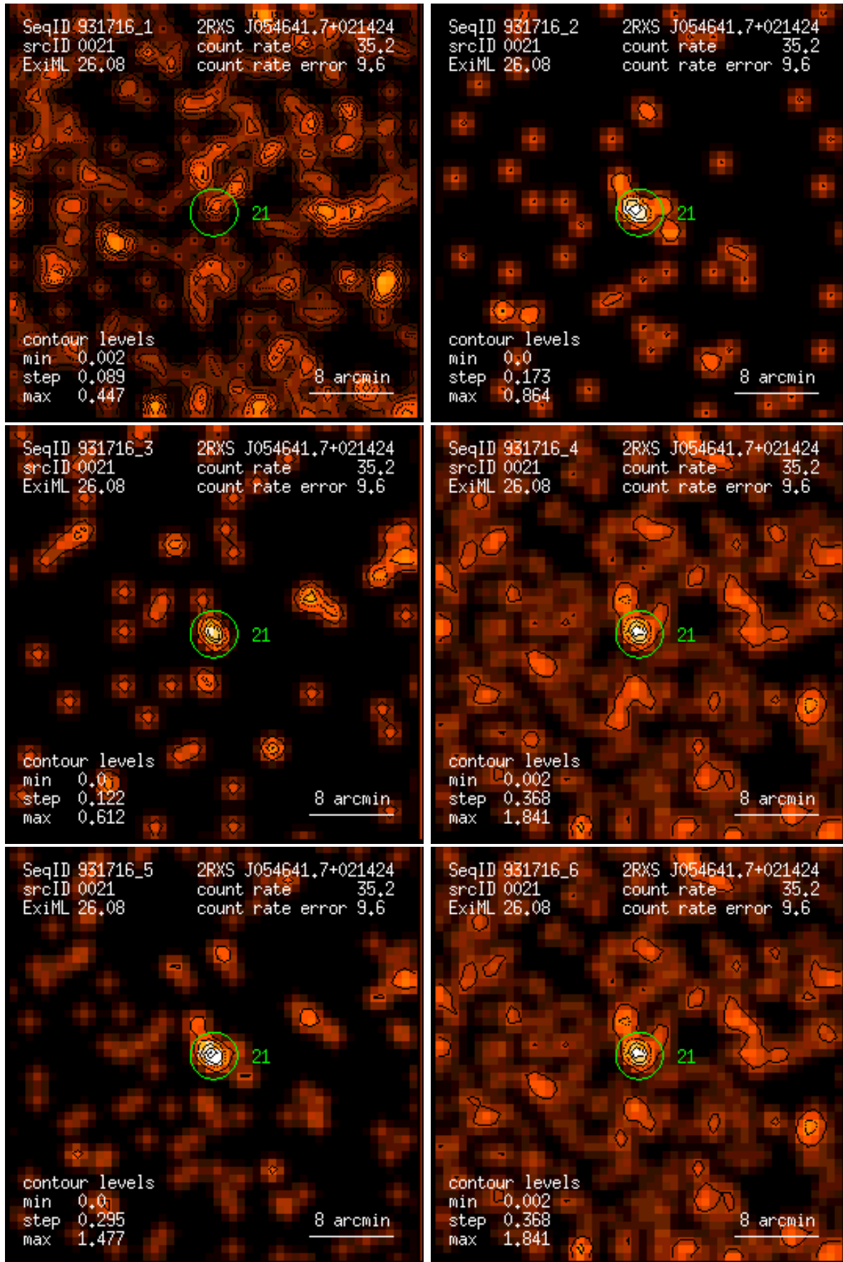
Figure 21: RASS 931716: detection 0021: band rate images, Gaussian filter: (1) PSPC channels 11 – 41, (2) 52 – 90, (3) 91 – 201, (4) 11 – 235, (5) 52 – 201, (6) 11 – 201. Broad band rates in counts/ks. Band rate contour levels in counts/ks/arcmin 2 .
