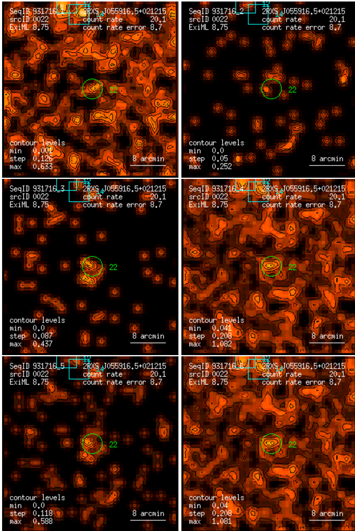
Figure 22: RASS 931716: detection 0022: band rate images, Gaussian filter: (1) PSPC channels 11 – 41, (2) 52 – 90, (3) 91 – 201, (4) 11 – 235, (5) 52 – 201, (6) 11 – 201. Broad band rates in counts/ks. Band rate contour levels in counts/ks/arcmin 2 .
