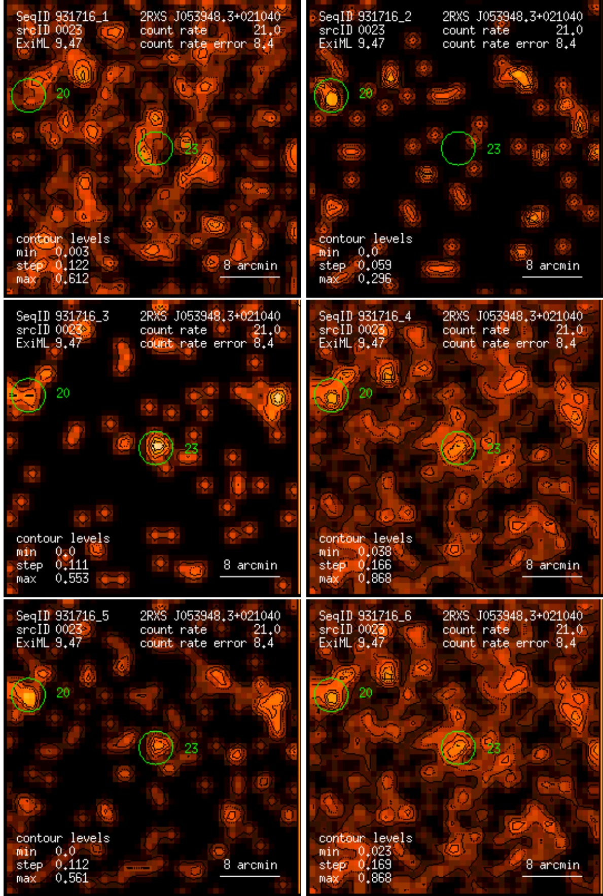
Figure 23: RASS 931716: detection 0023: band rate images, Gaussian filter: (1) PSPC channels 11 – 41, (2) 52 – 90, (3) 91 – 201, (4) 11 – 235, (5) 52 – 201, (6) 11 – 201. Broad band rates in counts/ks. Band rate contour levels in counts/ks/arcmin 2 .
