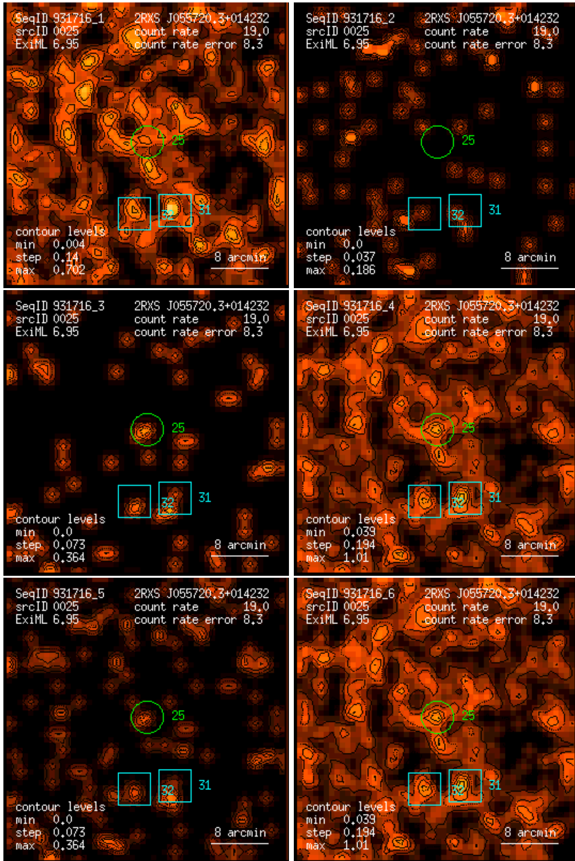
Figure 25: RASS 931716: detection 0025: band rate images, Gaussian filter: (1) PSPC channels 11 – 41, (2) 52 – 90, (3) 91 – 201, (4) 11 – 235, (5) 52 – 201, (6) 11 – 201. Broad band rates in counts/ks. Band rate contour levels in counts/ks/arcmin 2 .
