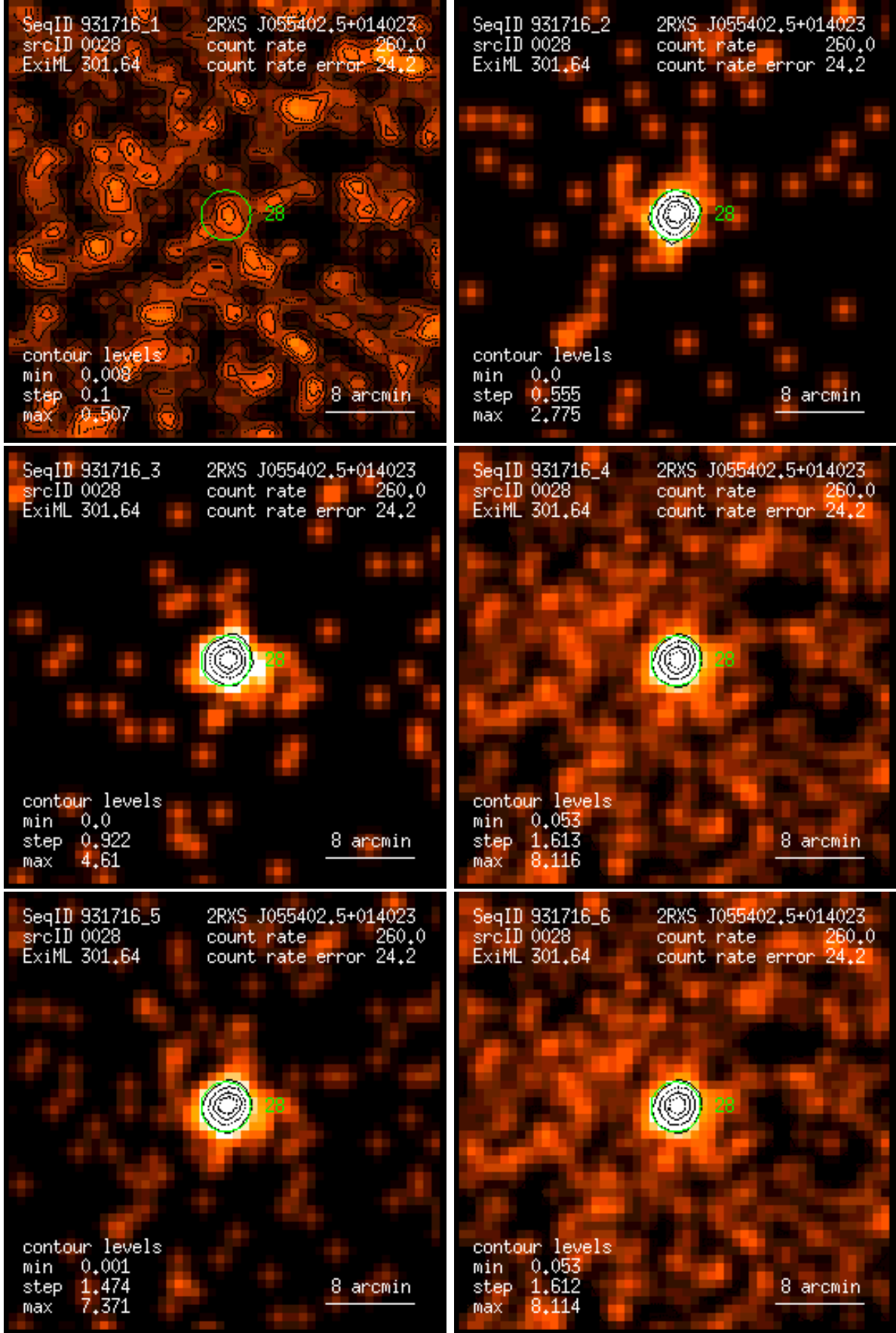
Figure 28: RASS 931716: detection 0028: band rate images, Gaussian filter: (1) PSPC channels 11 – 41, (2) 52 – 90, (3) 91 – 201, (4) 11 – 235, (5) 52 – 201, (6) 11 – 201. Broad band rates in counts/ks. Band rate contour levels in counts/ks/arcmin 2 .
