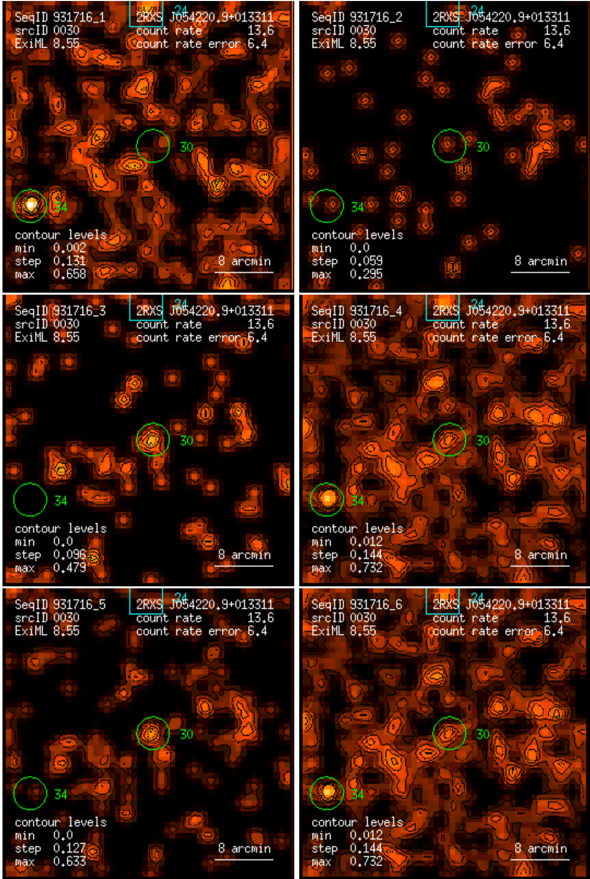
Figure 30: RASS 931716: detection 0030: band rate images, Gaussian filter: (1) PSPC channels 11 – 41, (2) 52 – 90, (3) 91 – 201, (4) 11 – 235, (5) 52 – 201, (6) 11 – 201. Broad band rates in counts/ks. Band rate contour levels in counts/ks/arcmin 2 .
