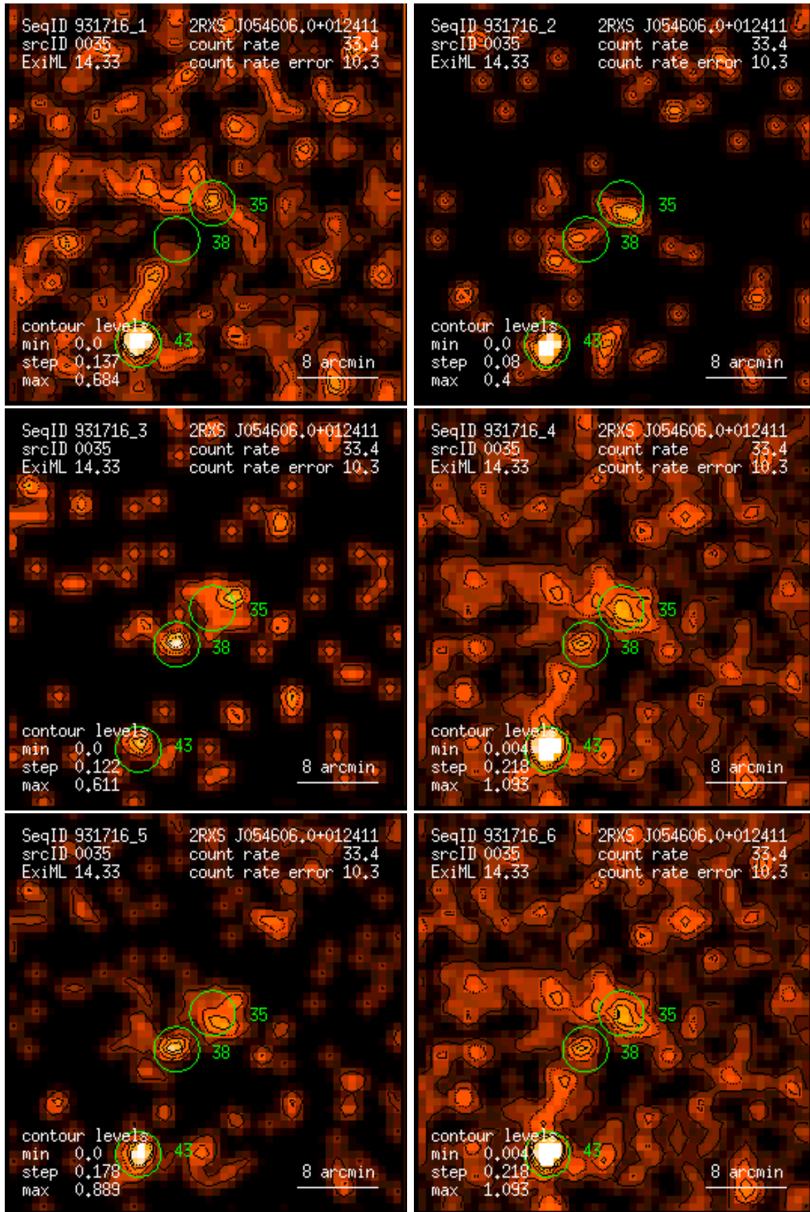
Figure 35: RASS 931716: detection 0035: band rate images, Gaussian filter: (1) PSPC channels 11 – 41, (2) 52 – 90, (3) 91 – 201, (4) 11 – 235, (5) 52 – 201, (6) 11 – 201. Broad band rates in counts/ks. Band rate contour levels in counts/ks/arcmin 2 .
