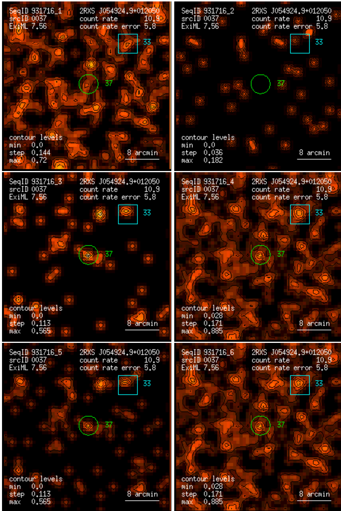
Figure 37: RASS 931716: detection 0037: band rate images, Gaussian filter: (1) PSPC channels 11 – 41, (2) 52 – 90, (3) 91 – 201, (4) 11 – 235, (5) 52 – 201, (6) 11 – 201. Broad band rates in counts/ks. Band rate contour levels in counts/ks/arcmin 2 .
