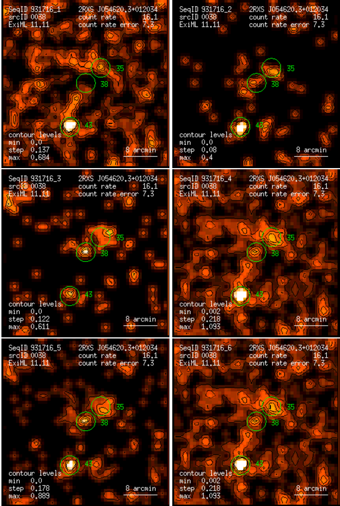
Figure 38: RASS 931716: detection 0038: band rate images, Gaussian filter: (1) PSPC channels 11 – 41, (2) 52 – 90, (3) 91 – 201, (4) 11 – 235, (5) 52 – 201, (6) 11 – 201. Broad band rates in counts/ks. Band rate contour levels in counts/ks/arcmin 2 .
