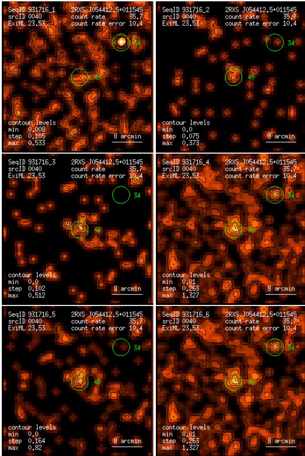
Figure 40: RASS 931716: detection 0040: band rate images, Gaussian filter: (1) PSPC channels 11 – 41, (2) 52 – 90, (3) 91 – 201, (4) 11 – 235, (5) 52 – 201, (6) 11 – 201. Broad band rates in counts/ks. Band rate contour levels in counts/ks/arcmin 2 .
