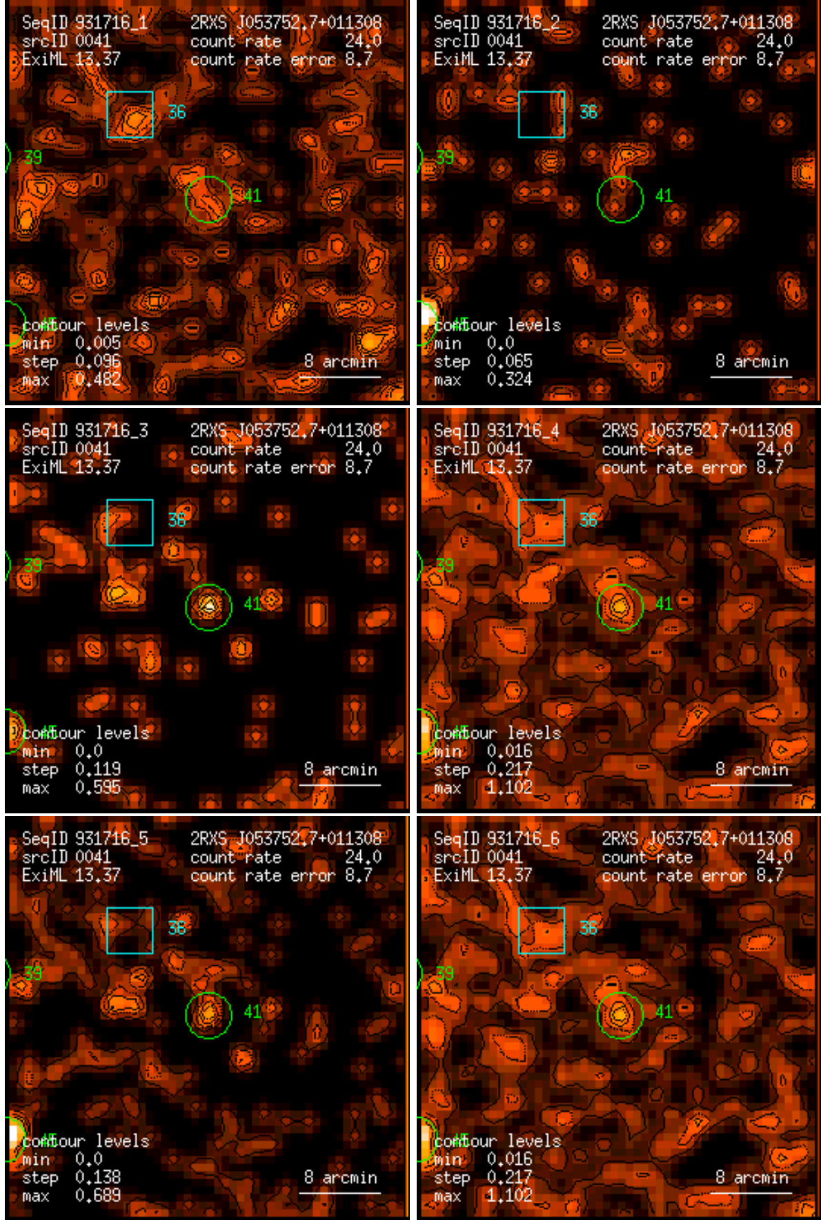
Figure 41: RASS 931716: detection 0041: band rate images, Gaussian filter: (1) PSPC channels 11 – 41, (2) 52 – 90, (3) 91 – 201, (4) 11 – 235, (5) 52 – 201, (6) 11 – 201. Broad band rates in counts/ks. Band rate contour levels in counts/ks/arcmin 2 .
