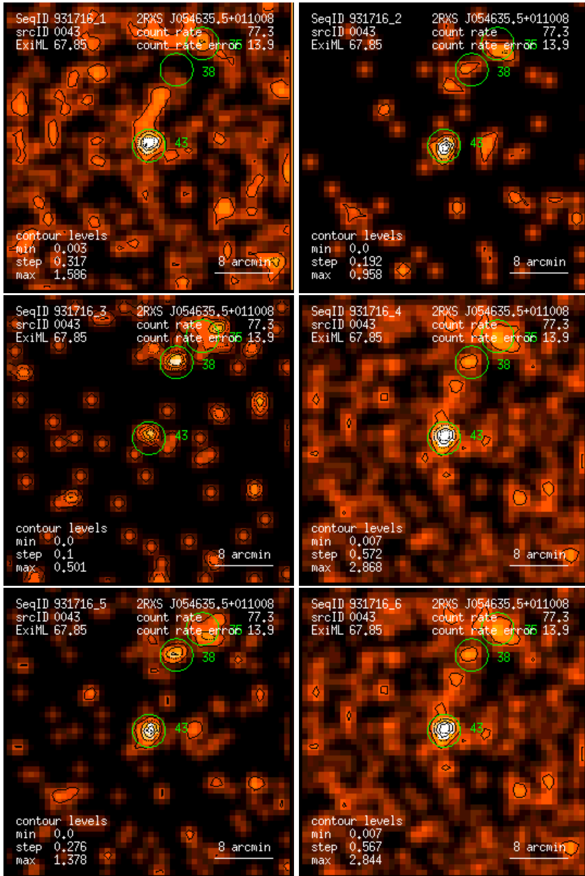
Figure 43: RASS 931716: detection 0043: band rate images, Gaussian filter: (1) PSPC channels 11 – 41, (2) 52 – 90, (3) 91 – 201, (4) 11 – 235, (5) 52 – 201, (6) 11 – 201. Broad band rates in counts/ks. Band rate contour levels in counts/ks/arcmin 2 .
