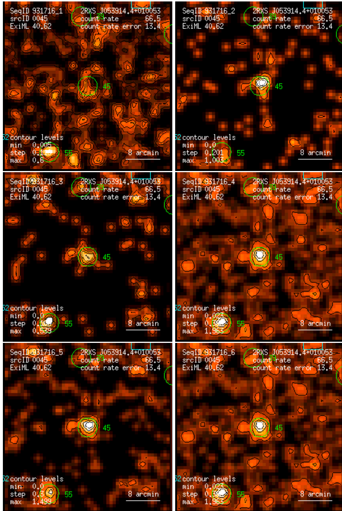
Figure 45: RASS 931716: detection 0045: band rate images, Gaussian filter: (1) PSPC channels 11 – 41, (2) 52 – 90, (3) 91 – 201, (4) 11 – 235, (5) 52 – 201, (6) 11 – 201. Broad band rates in counts/ks. Band rate contour levels in counts/ks/arcmin 2 .
