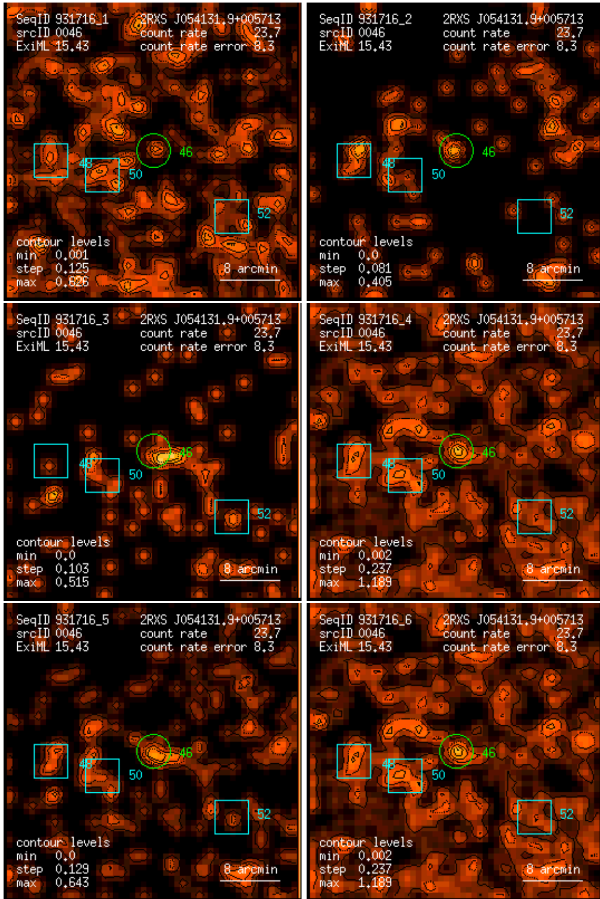
Figure 46: RASS 931716: detection 0046: band rate images, Gaussian filter: (1) PSPC channels 11 – 41, (2) 52 – 90, (3) 91 – 201, (4) 11 – 235, (5) 52 – 201, (6) 11 – 201. Broad band rates in counts/ks. Band rate contour levels in counts/ks/arcmin 2 .
