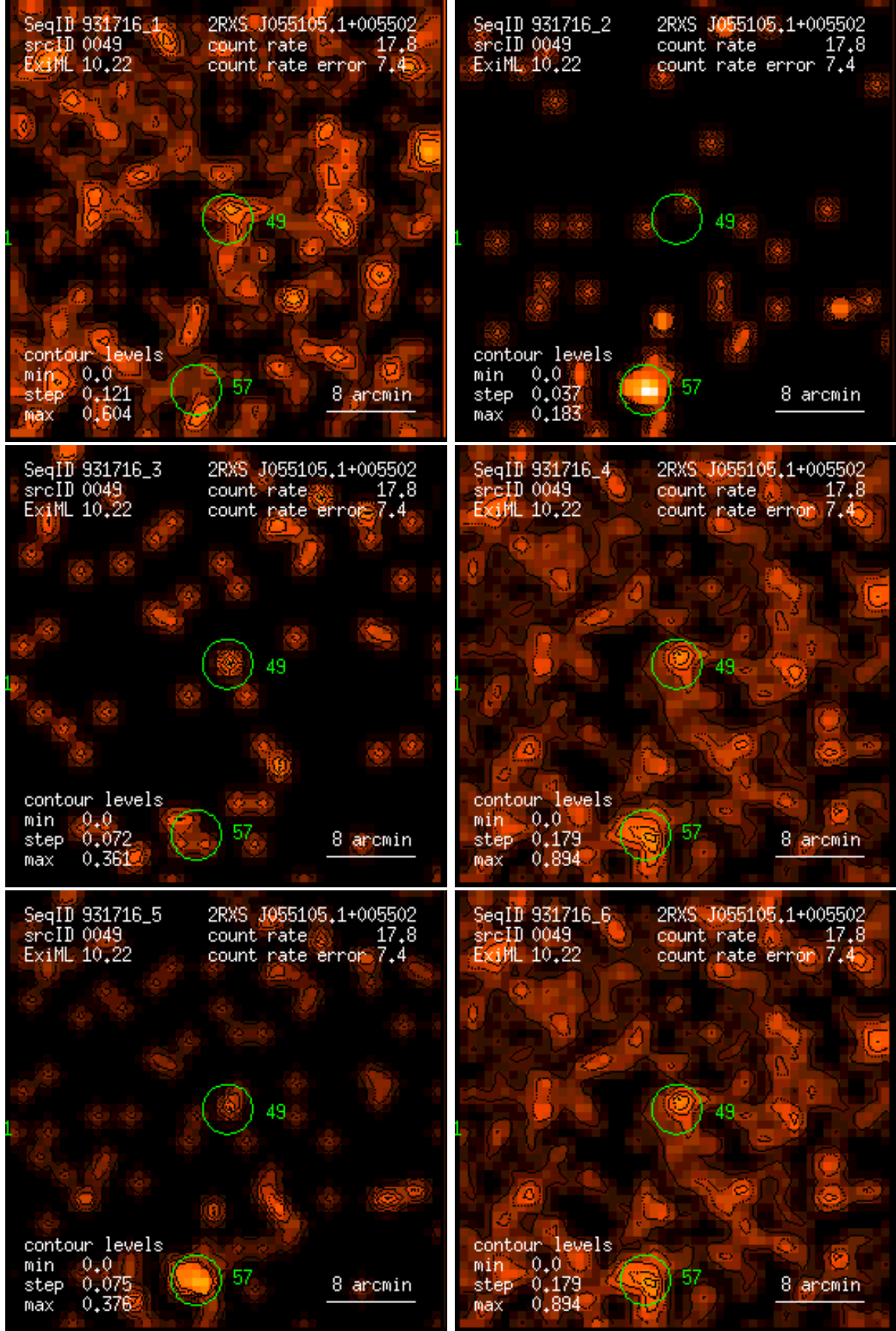
Figure 49: RASS 931716: detection 0049: band rate images, Gaussian filter: (1) PSPC channels 11 – 41, (2) 52 – 90, (3) 91 – 201, (4) 11 – 235, (5) 52 – 201, (6) 11 – 201. Broad band rates in counts/ks. Band rate contour levels in counts/ks/arcmin 2 .
