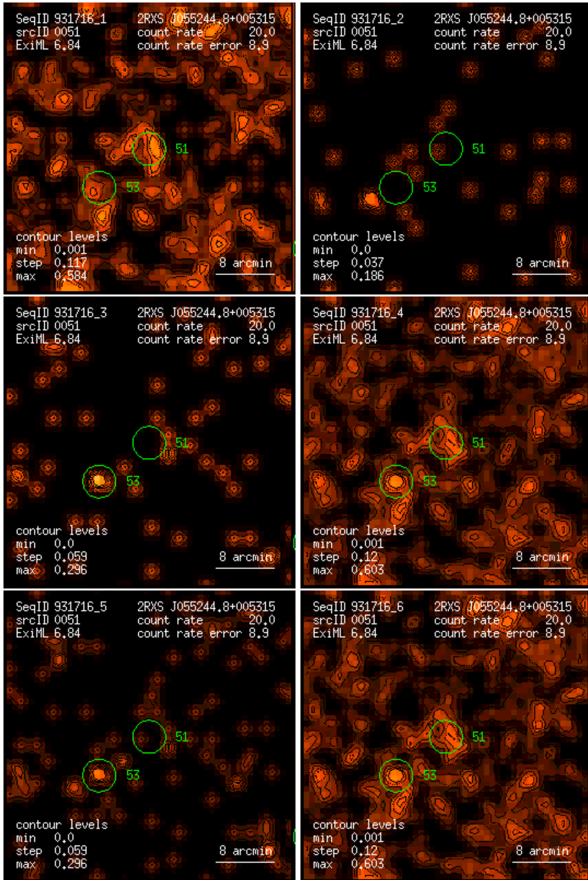
Figure 51: RASS 931716: detection 0051: band rate images, Gaussian filter: (1) PSPC channels 11 – 41, (2) 52 – 90, (3) 91 – 201, (4) 11 – 235, (5) 52 – 201, (6) 11 – 201. Broad band rates in counts/ks. Band rate contour levels in counts/ks/arcmin 2 .
