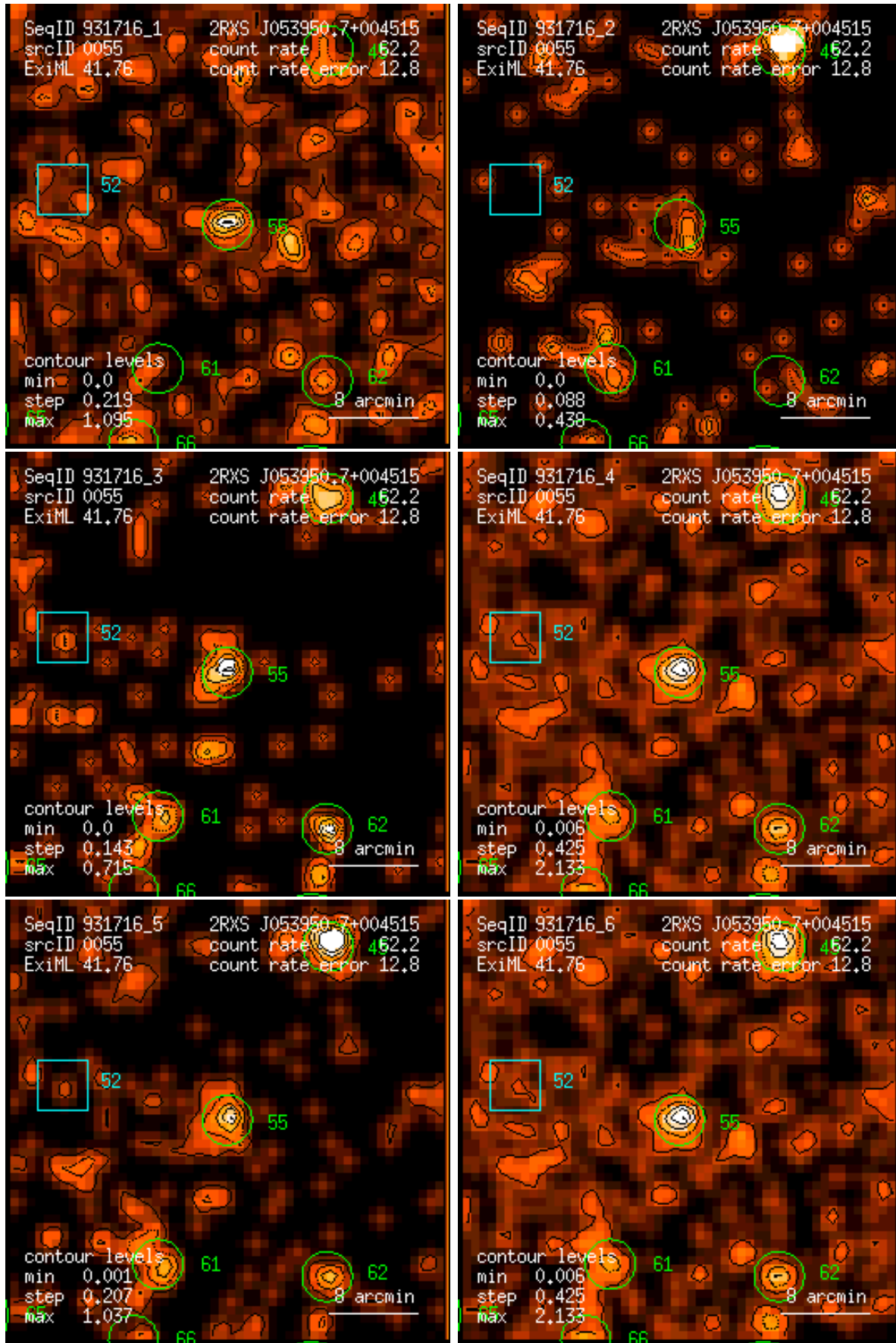
Figure 55: RASS 931716: detection 0055: band rate images, Gaussian filter: (1) PSPC channels 11 – 41, (2) 52 – 90, (3) 91 – 201, (4) 11 – 235, (5) 52 – 201, (6) 11 – 201. Broad band rates in counts/ks. Band rate contour levels in counts/ks/arcmin 2 .
