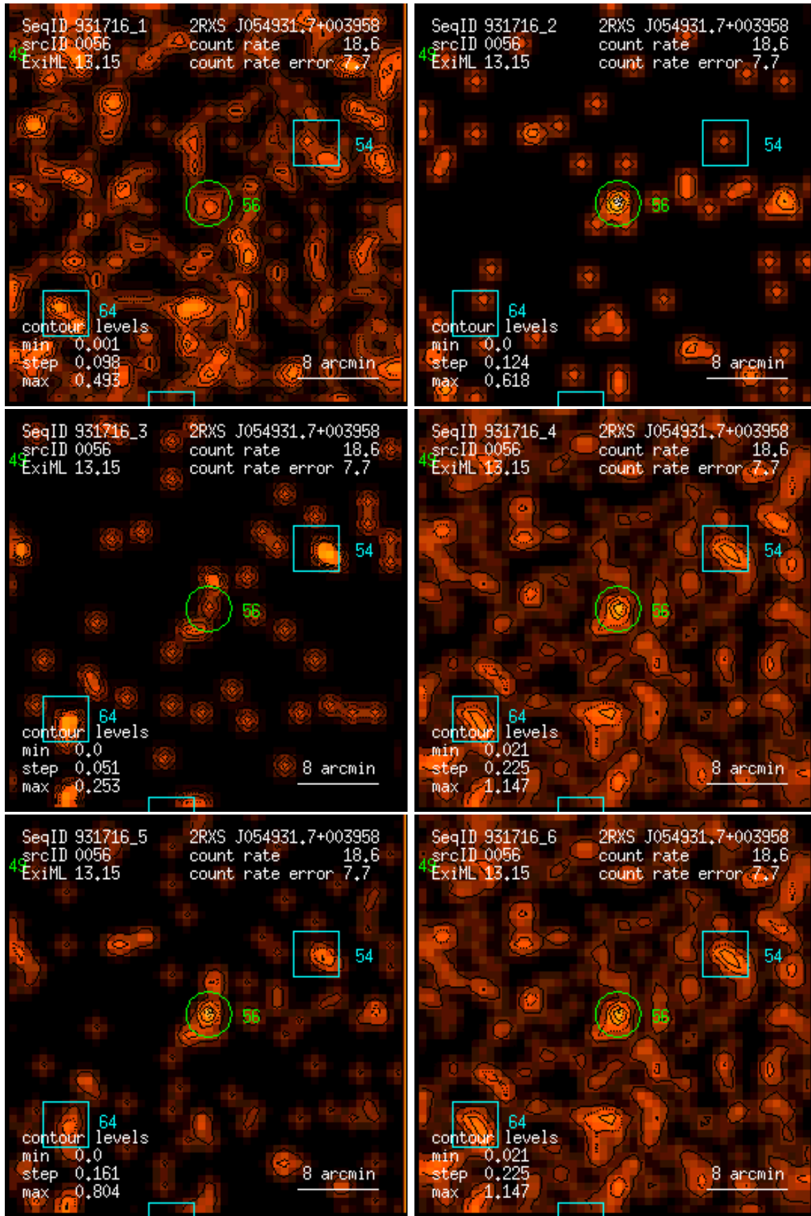
Figure 56: RASS 931716: detection 0056: band rate images, Gaussian filter: (1) PSPC channels 11 – 41, (2) 52 – 90, (3) 91 – 201, (4) 11 – 235, (5) 52 – 201, (6) 11 – 201. Broad band rates in counts/ks. Band rate contour levels in counts/ks/arcmin 2 .
