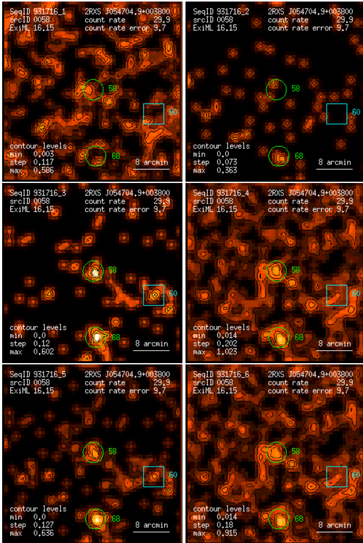
Figure 58: RASS 931716: detection 0058: band rate images, Gaussian filter: (1) PSPC channels 11 – 41, (2) 52 – 90, (3) 91 – 201, (4) 11 – 235, (5) 52 – 201, (6) 11 – 201. Broad band rates in counts/ks. Band rate contour levels in counts/ks/arcmin 2 .
