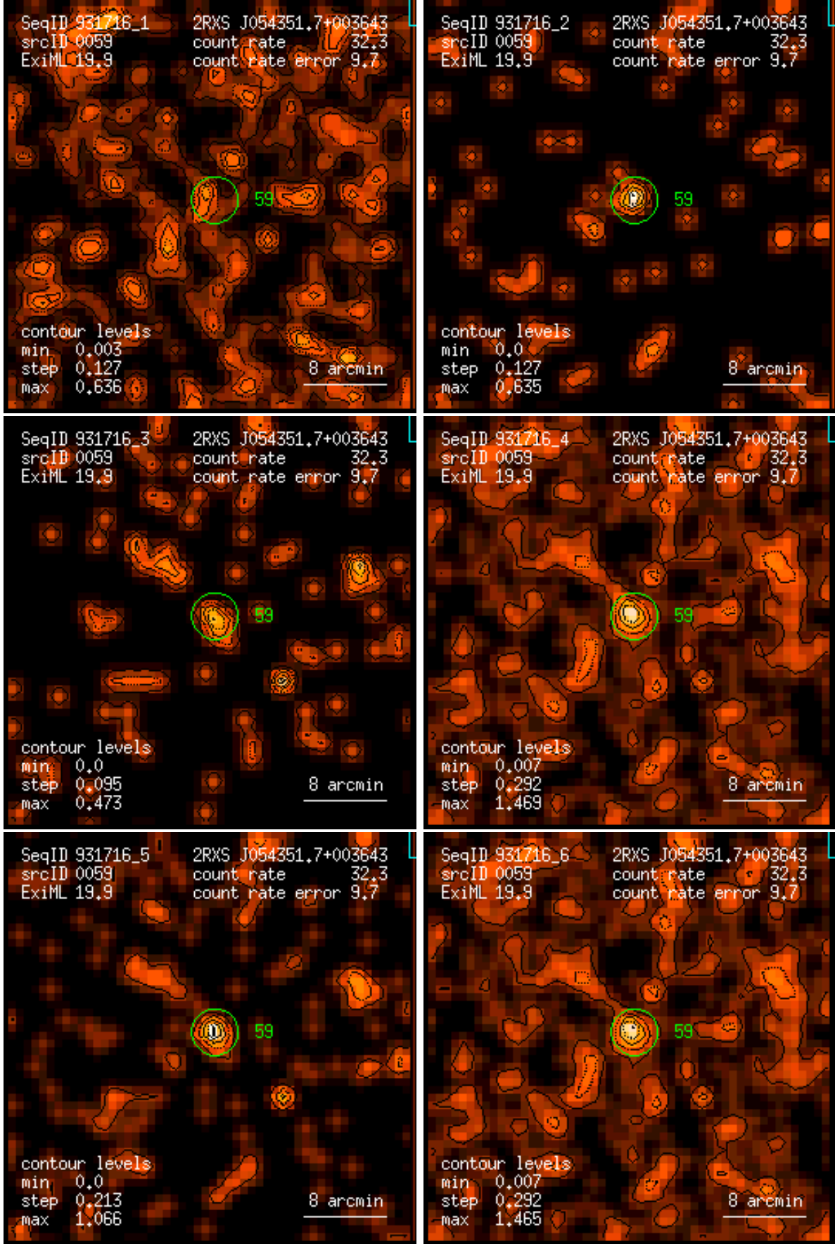
Figure 59: RASS 931716: detection 0059: band rate images, Gaussian filter: (1) PSPC channels 11 – 41, (2) 52 – 90, (3) 91 – 201, (4) 11 – 235, (5) 52 – 201, (6) 11 – 201. Broad band rates in counts/ks. Band rate contour levels in counts/ks/arcmin 2 .
