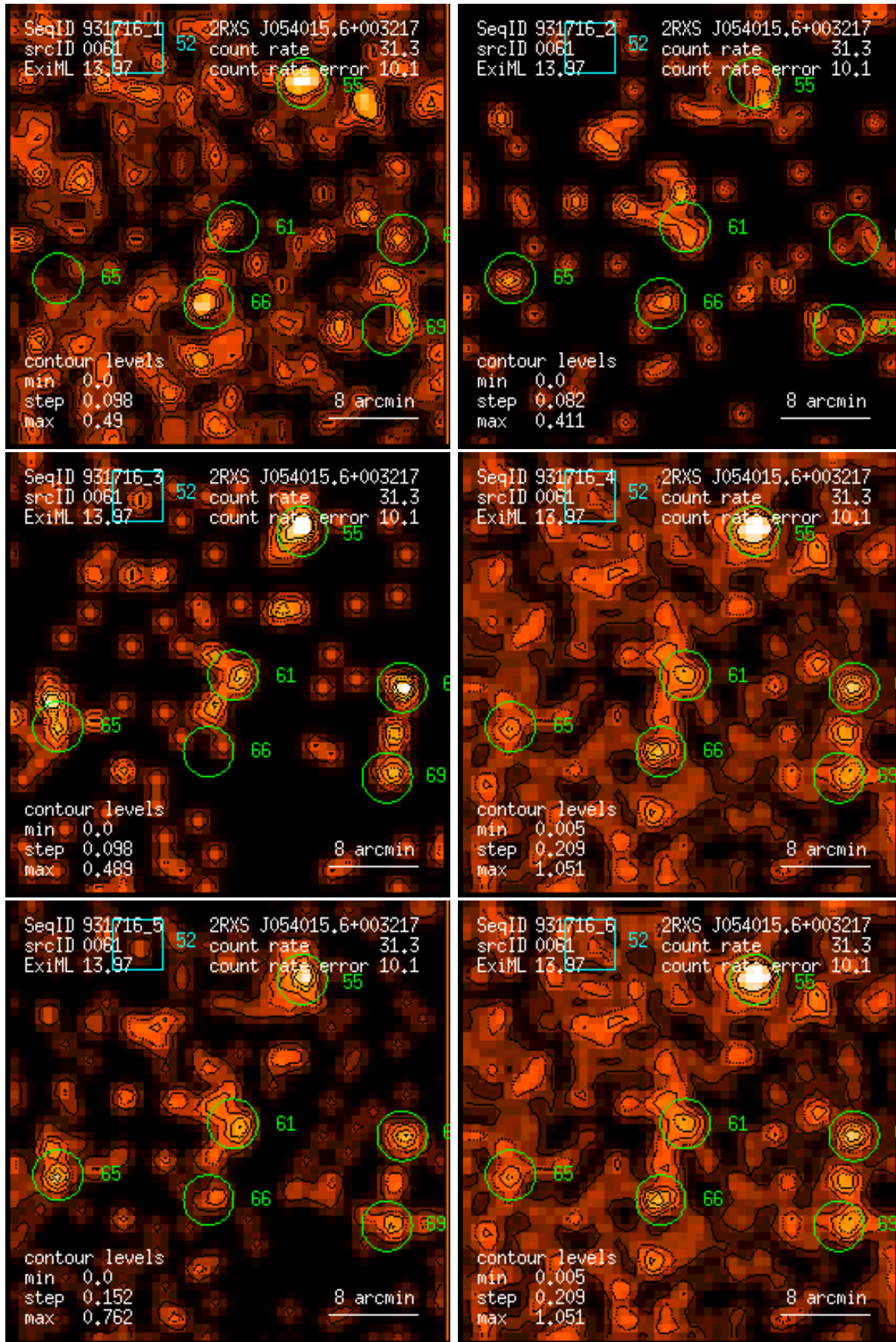
Figure 61: RASS 931716: detection 0061: band rate images, Gaussian filter: (1) PSPC channels 11 – 41, (2) 52 – 90, (3) 91 – 201, (4) 11 – 235, (5) 52 – 201, (6) 11 – 201. Broad band rates in counts/ks. Band rate contour levels in counts/ks/arcmin 2 .
