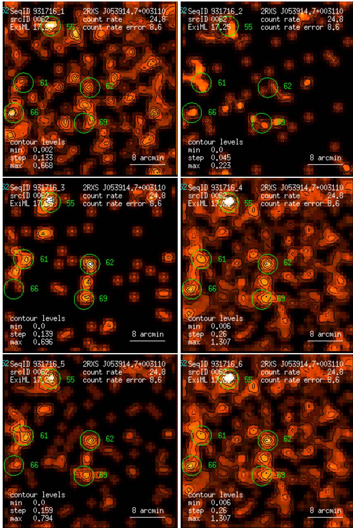
Figure 62: RASS 931716: detection 0062: band rate images, Gaussian filter: (1) PSPC channels 11 – 41, (2) 52 – 90, (3) 91 – 201, (4) 11 – 235, (5) 52 – 201, (6) 11 – 201. Broad band rates in counts/ks. Band rate contour levels in counts/ks/arcmin 2 .
