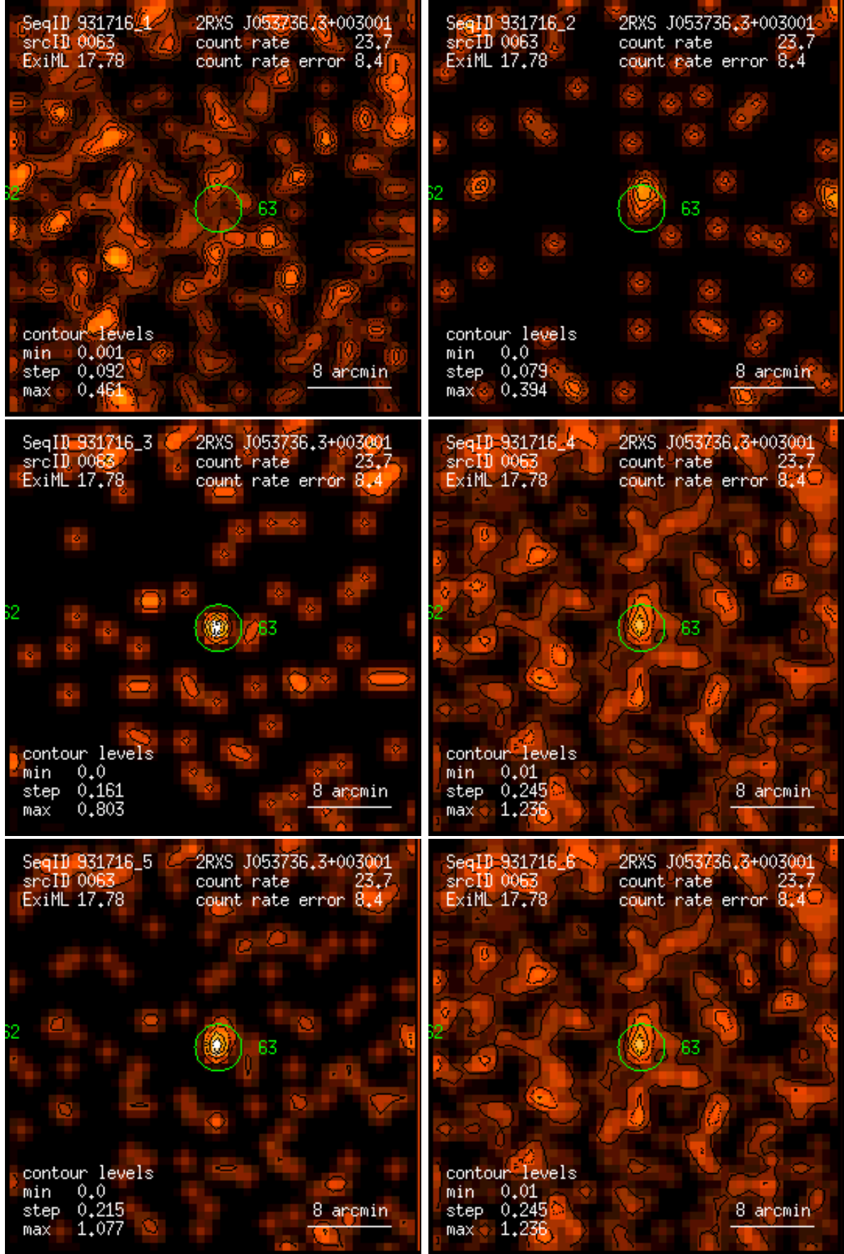
Figure 63: RASS 931716: detection 0063: band rate images, Gaussian filter: (1) PSPC channels 11 – 41, (2) 52 – 90, (3) 91 – 201, (4) 11 – 235, (5) 52 – 201, (6) 11 – 201. Broad band rates in counts/ks. Band rate contour levels in counts/ks/arcmin 2 .
