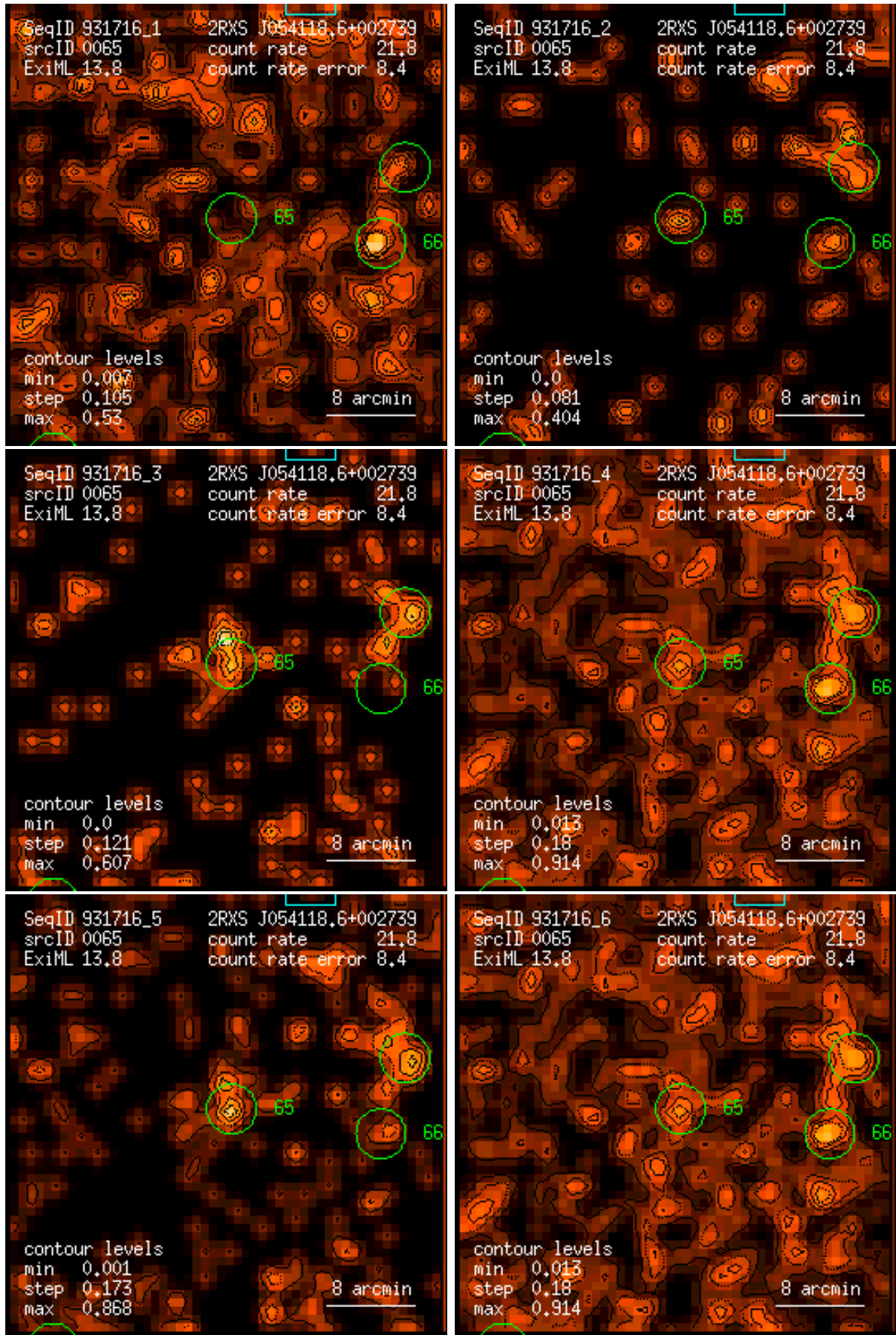
Figure 65: RASS 931716: detection 0065: band rate images, Gaussian filter: (1) PSPC channels 11 – 41, (2) 52 – 90, (3) 91 – 201, (4) 11 – 235, (5) 52 – 201, (6) 11 – 201. Broad band rates in counts/ks. Band rate contour levels in counts/ks/arcmin 2 .
