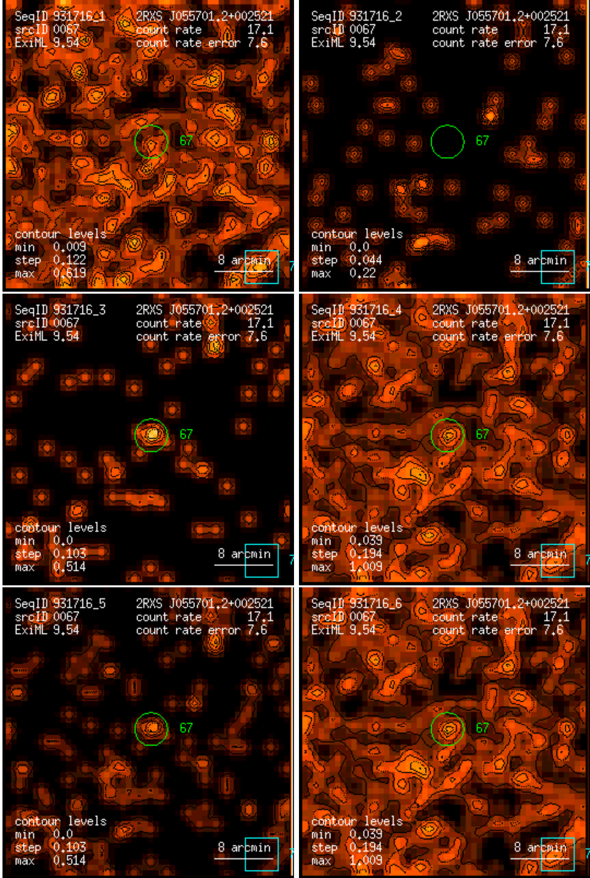
Figure 67: RASS 931716: detection 0067: band rate images, Gaussian filter: (1) PSPC channels 11 – 41, (2) 52 – 90, (3) 91 – 201, (4) 11 – 235, (5) 52 – 201, (6) 11 – 201. Broad band rates in counts/ks. Band rate contour levels in counts/ks/arcmin 2 .
