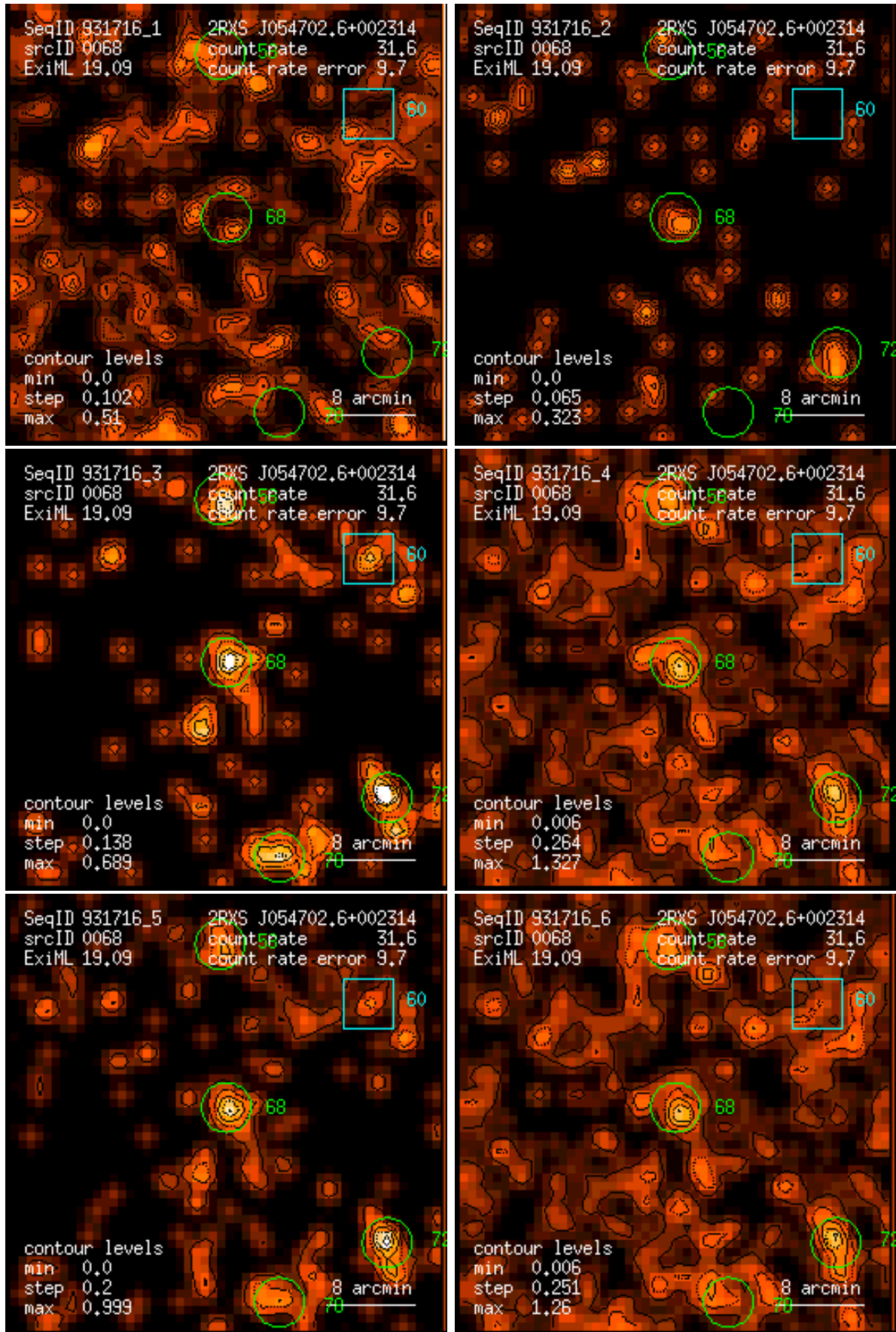
Figure 68: RASS 931716: detection 0068: band rate images, Gaussian filter: (1) PSPC channels 11 – 41, (2) 52 – 90, (3) 91 – 201, (4) 11 – 235, (5) 52 – 201, (6) 11 – 201. Broad band rates in counts/ks. Band rate contour levels in counts/ks/arcmin 2 .
